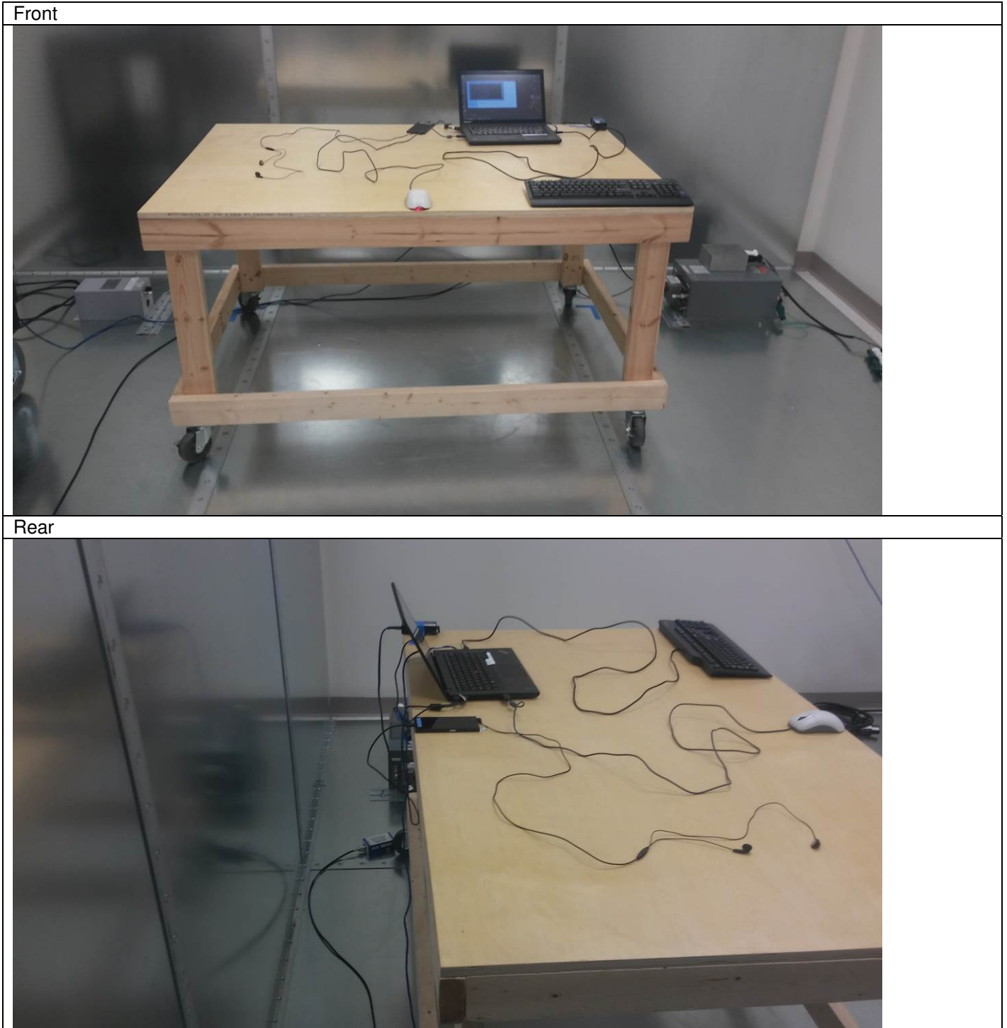
Figure 2 Test Setup for Conducted Emissions -Sync
