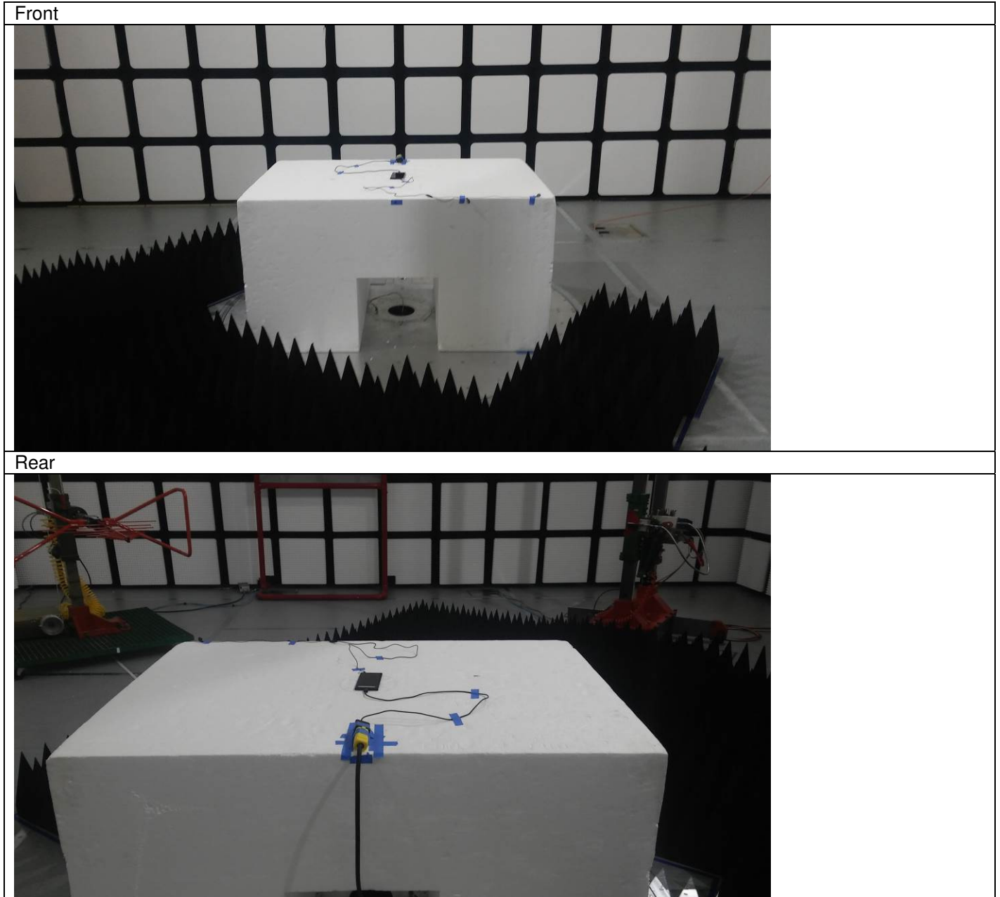
Figure 9 Test setup for Radiated Emissions > 1GHz Charger
