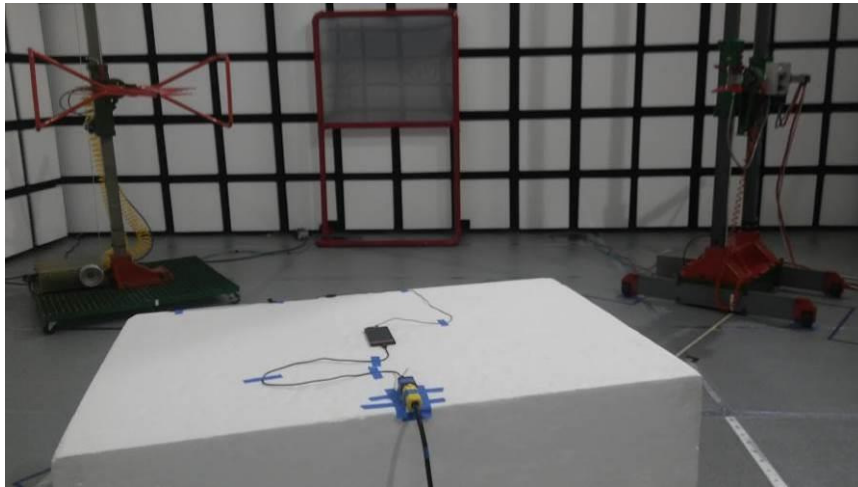
RADIATED EMISSIONS ABOVE 30 MHz (REAR)
