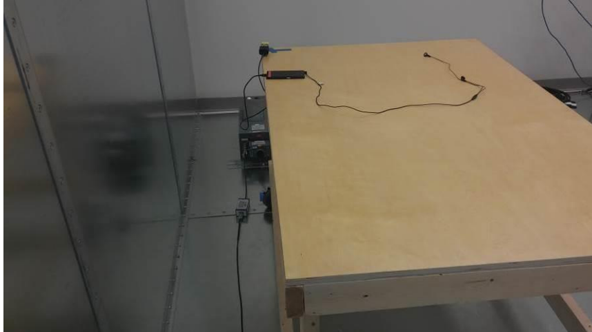
LINE CONDUCTED EMISSION (REAR)
