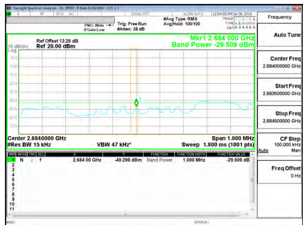
LTE B41 5MHz QPSK High Channel 1RB at 2.684GHz
