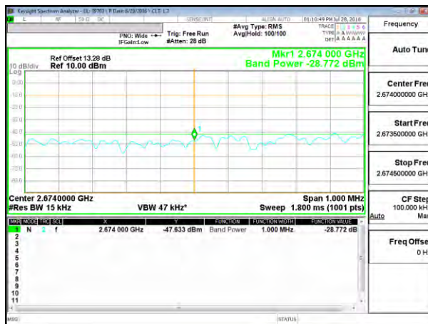
LTE B41 15MHz QPSK High Channel 1RB at 2.674 GHz
