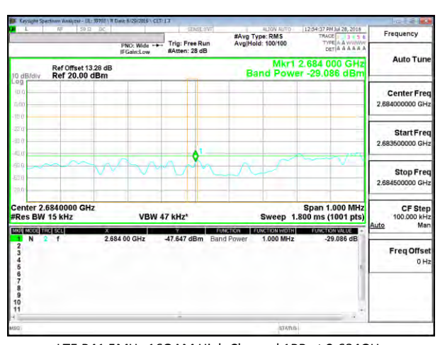
LTE B41 5MHz 16QAM High Channel 1RB at 2.684GHz
