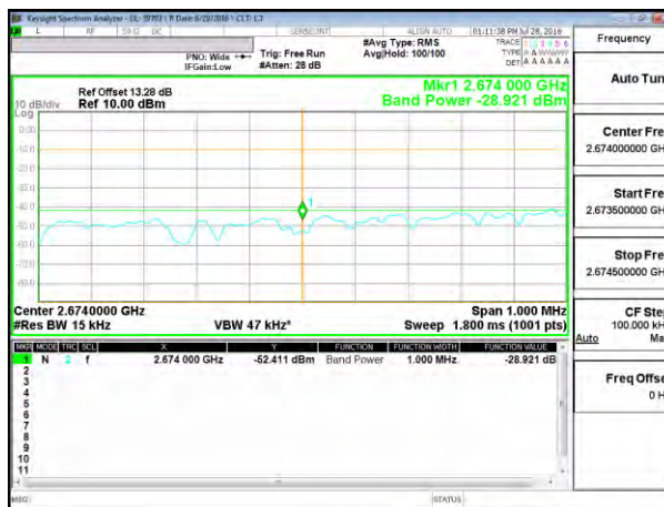
LTE B41 15MHz 16QAM High Channel 1RB 2.674 GHz
