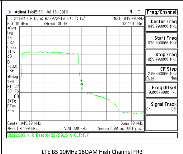
LTE B5 10MHz 16QAM High Channel FRB
