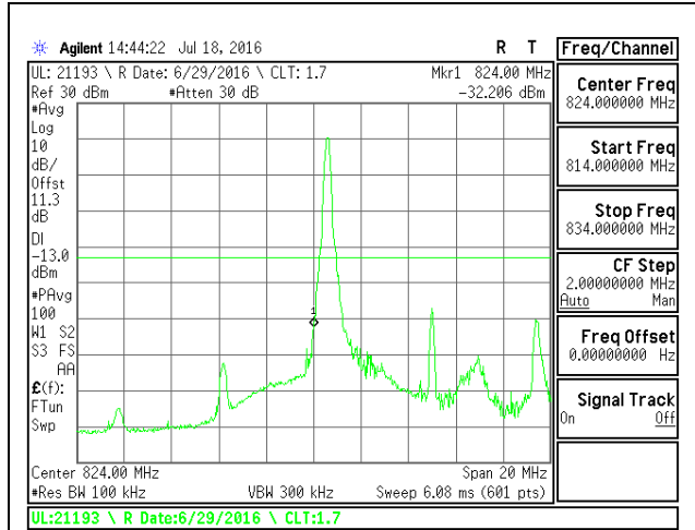
LTE B5 10MHz 16QAM Low Channel 1RB
