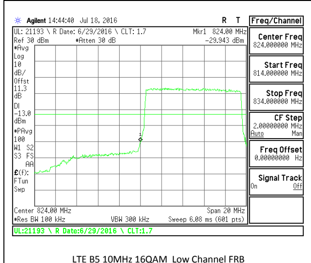
LTE B5 10MHz 16QAM Low Channel FRB
