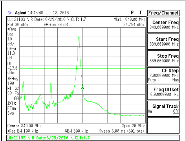
LTE B5 10MHz 16QAM High Channel 1RB
