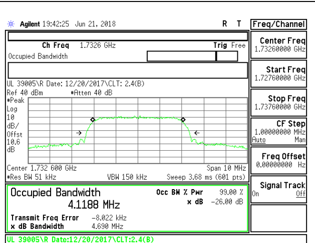
WCDMA BAND4 HSDPA MID Channel
