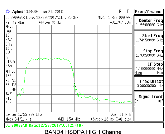
BAND4 HSDPA HIGH Channel
