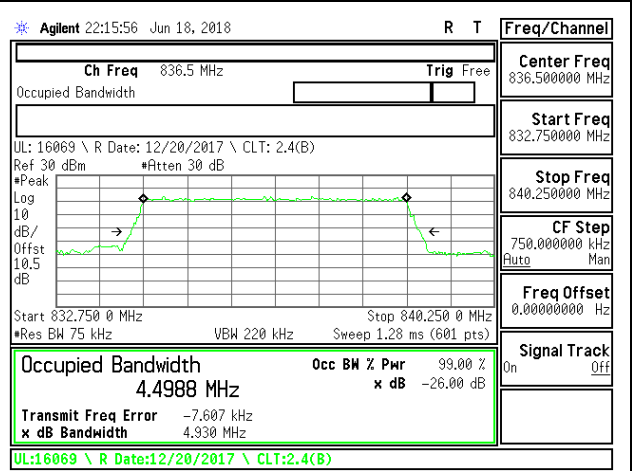
LTE B5 5MHz 16QAM Mid Channel RB25-0
