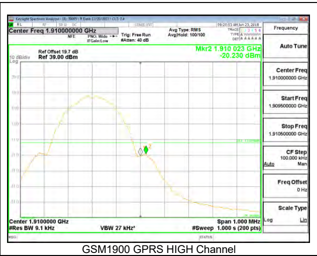
GSM1900 GPRS HIGH Channel
