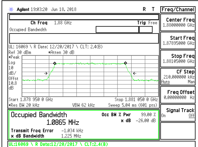
LTE B2 1.4MHz QPSK Mid Channel RB6-0
