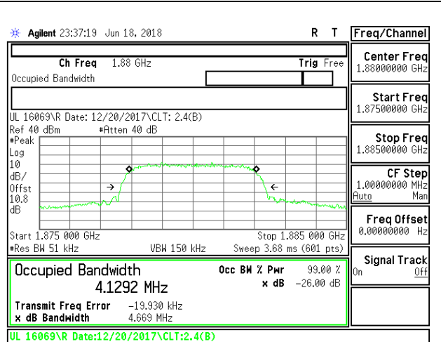
WCDMA BAND2 HSDPA MID Channel
