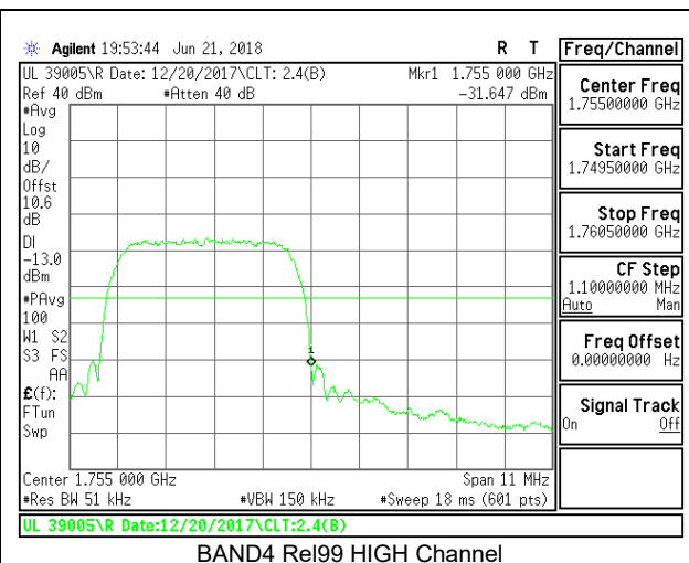
BAND4 Rel99 HIGH Channel
