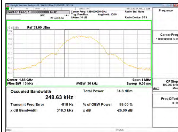
GSM 1900MHz GPRS MID Channel
