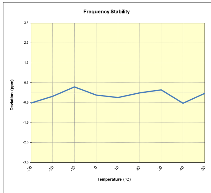
Plot 7-34. LTE Band 41(PC3) Frequency Stability Chart
