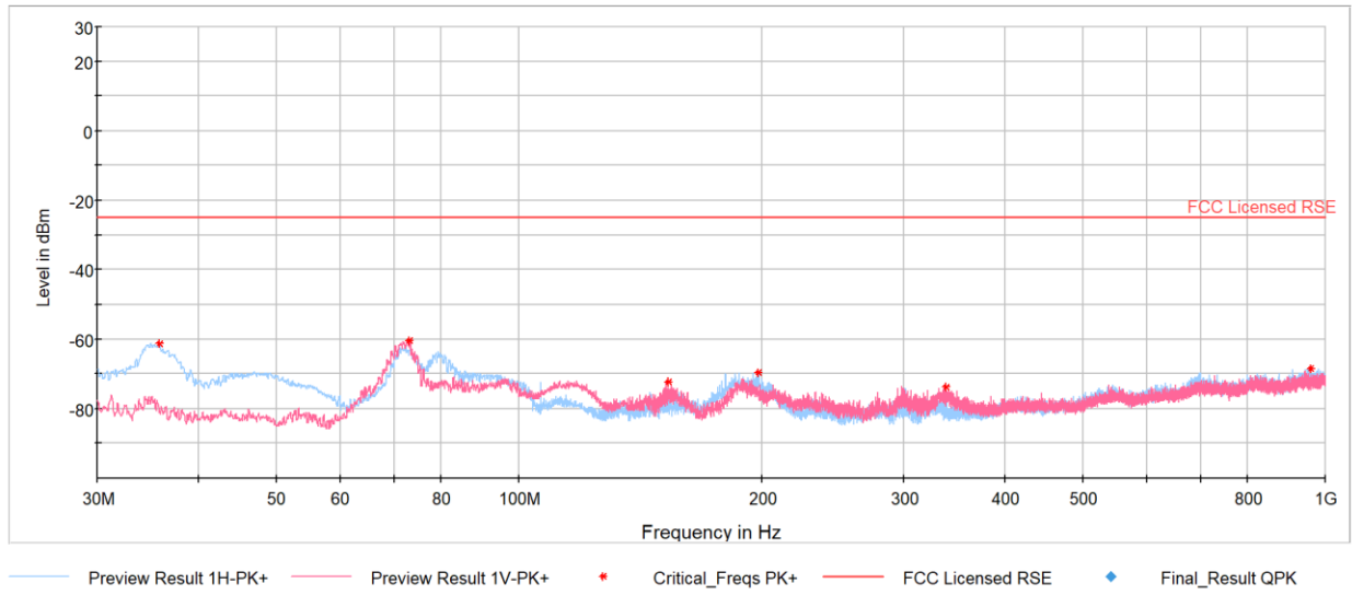
Plot 7-30. Radiated Spurious Plot Below 1GHz (LTE Band 41(PC3))
