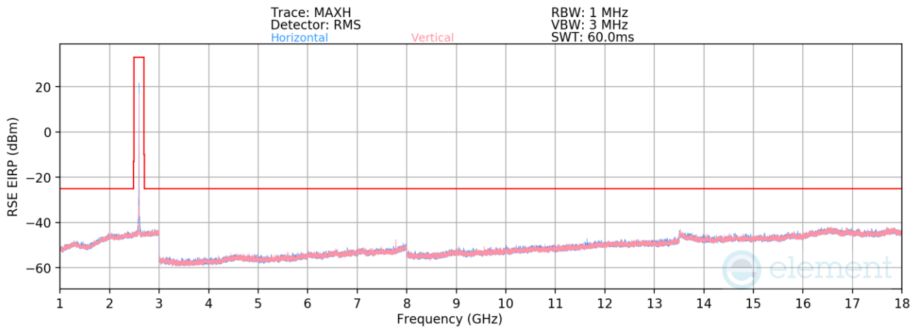
Plot 7-31. Radiated Spurious Plot (LTE Band 41(PC3))
