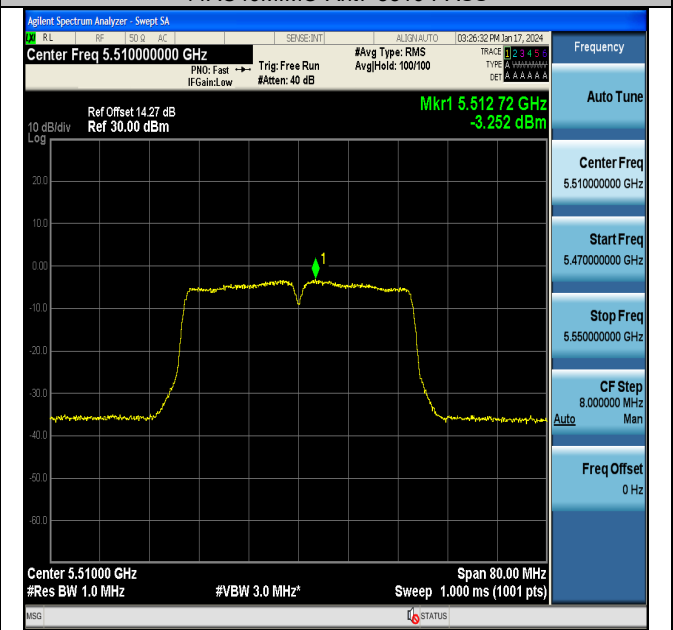
11AC40MIMO-Ant7-5510-PASS
