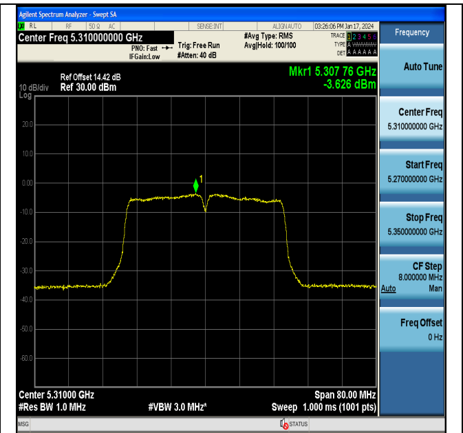
11AC40MIMO-Ant7-5310-PASS
