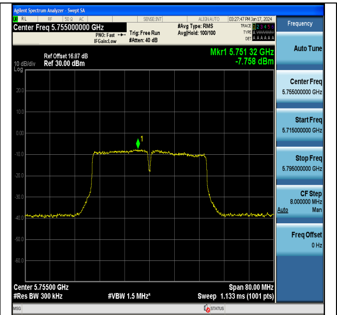
11AC40MIMO-Ant7-5755-PASS
