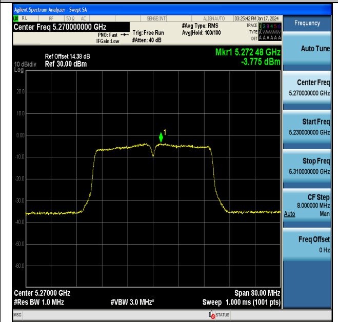
11AC40MIMO-Ant7-5270-PASS
