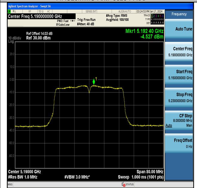
11AC40MIMO-Ant7-5190-PASS
