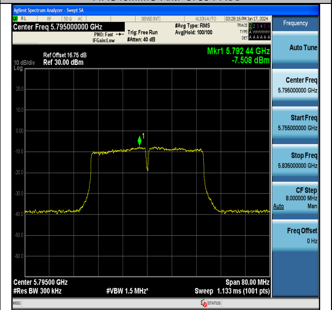
11AC40MIMO-Ant7-5795-PASS
