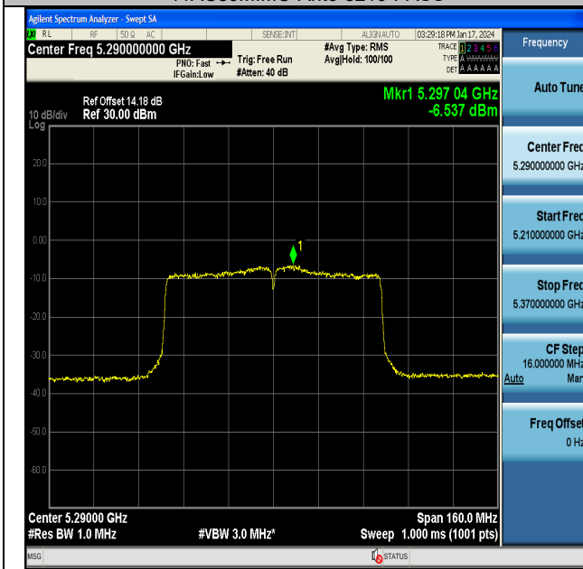
11AC80MIMO-Ant6-5290-PASS
