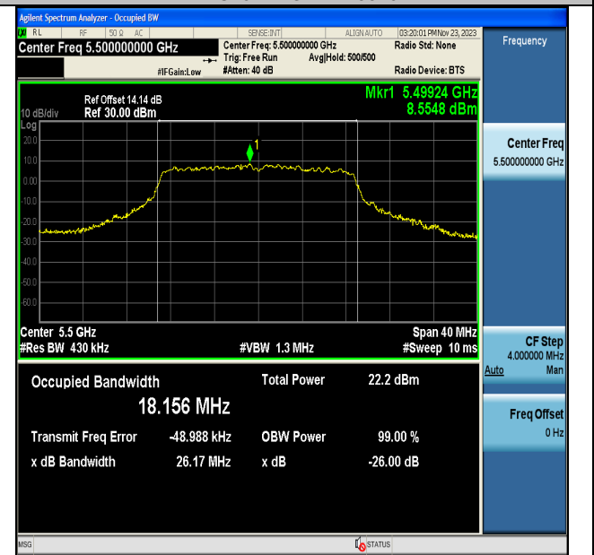
11AC20MIMO-Ant7-5500
