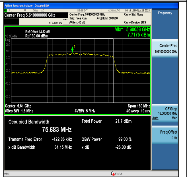
11AC80MIMO-Ant7-5610
