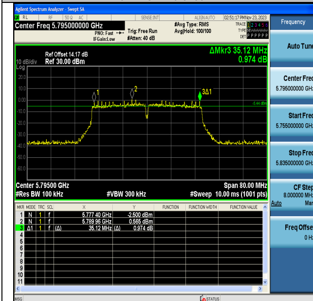
11N40MIMO-Ant6-5795-PASS
