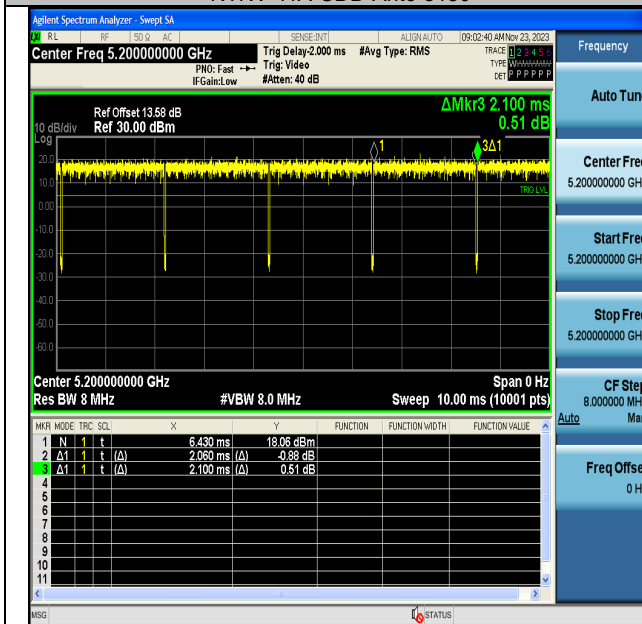
NTVN-11A-CDD-Ant6-5200
