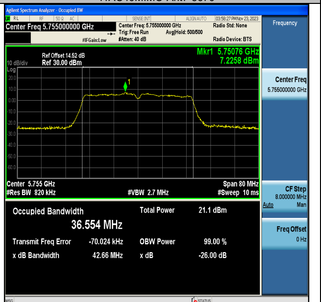
11AC40MIMO-Ant7-5755
