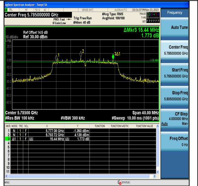
11AC20MIMO-Ant7-5785-PASS
