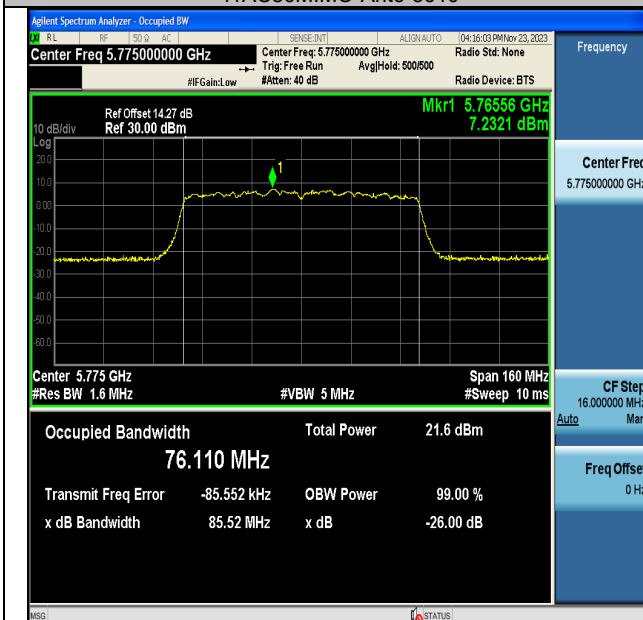
11AC80MIMO-Ant6-5775
