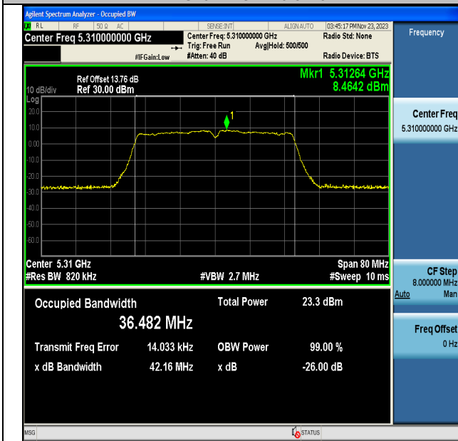
11AC40MIMO-Ant6-5310
