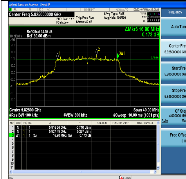
11AC20MIMO-Ant6-5825-PASS
