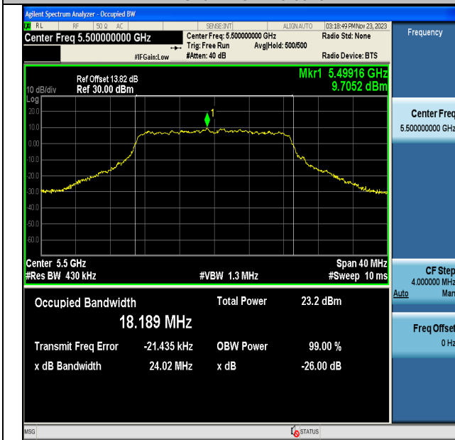
11AC20MIMO-Ant6-5500
