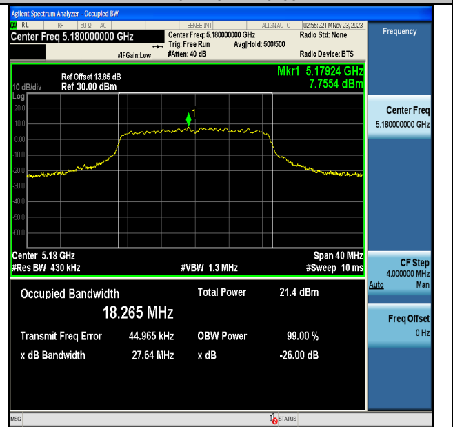
11A20MIMO-Ant7-5180
