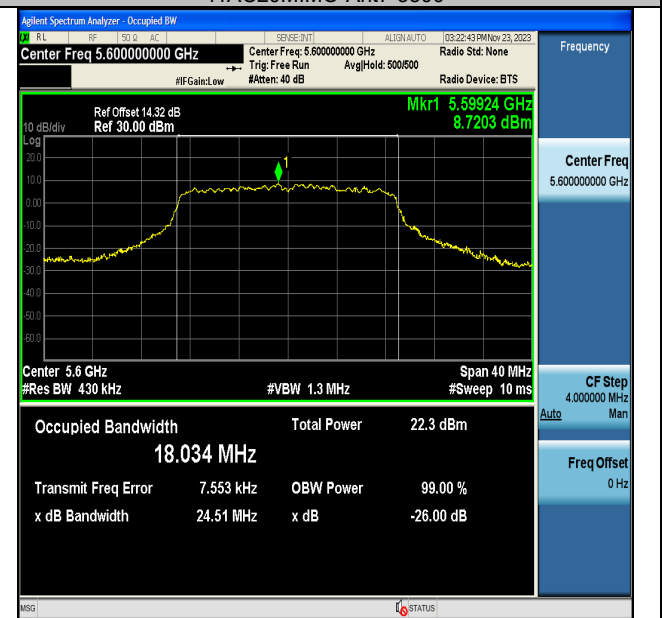
11AC20MIMO-Ant7-5600
