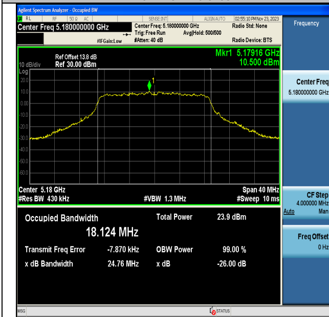
11A20MIMO-Ant6-5180
