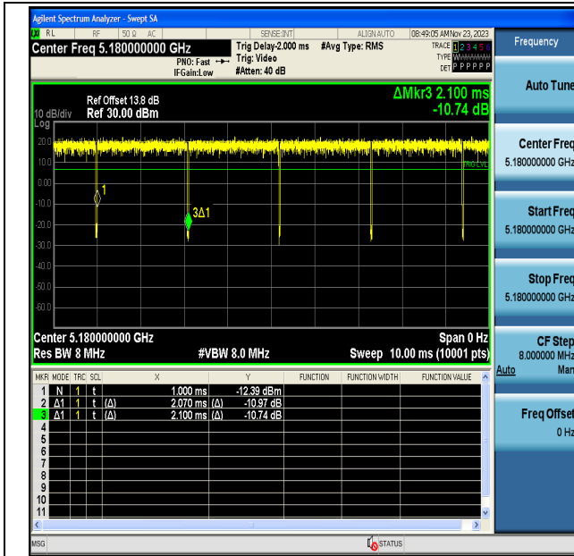
NTVN-11A-CDD-Ant6-5180
