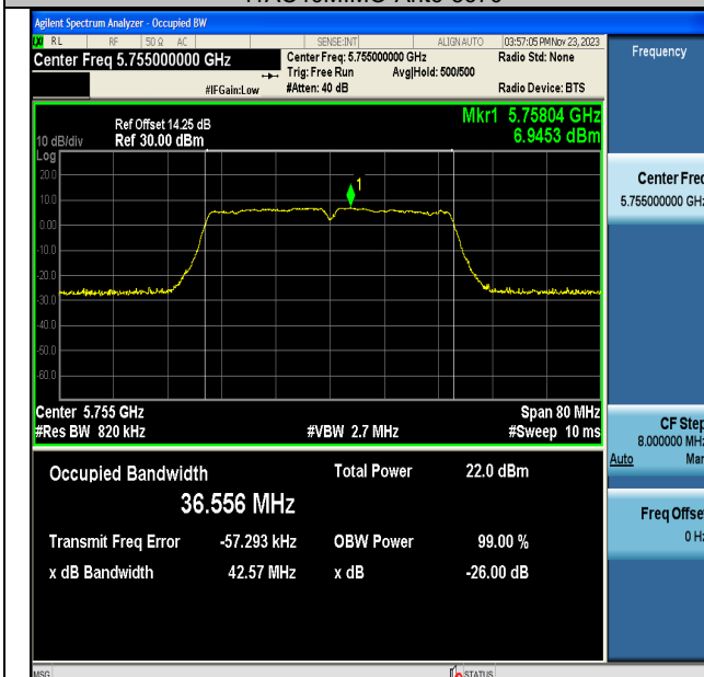
11AC40MIMO-Ant6-5755
