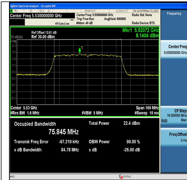
11AC80MIMO-Ant6-5530
