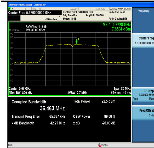
11AC40MIMO-Ant6-5670
