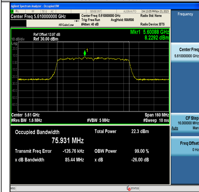
11AC80MIMO-Ant6-5610
