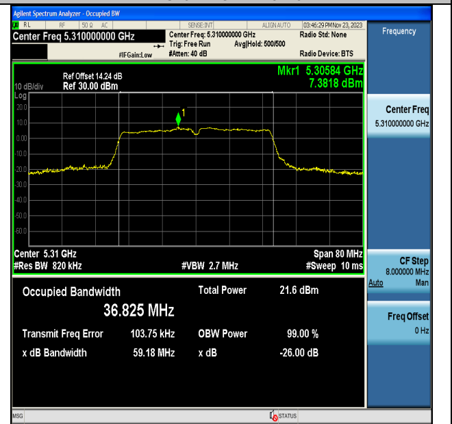
11AC40MIMO-Ant7-5310
