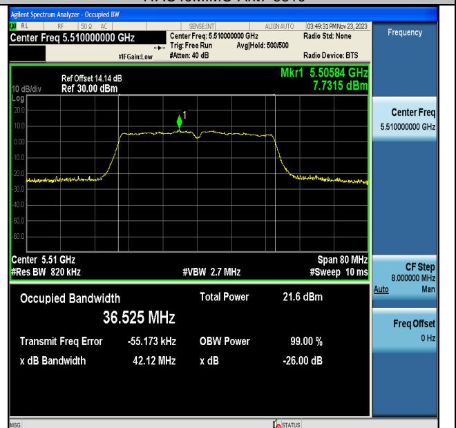
11AC40MIMO-Ant7-5510
