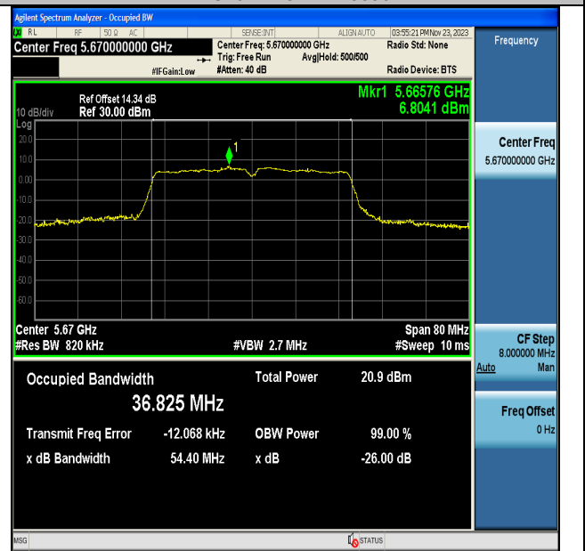
11AC40MIMO-Ant7-5670
