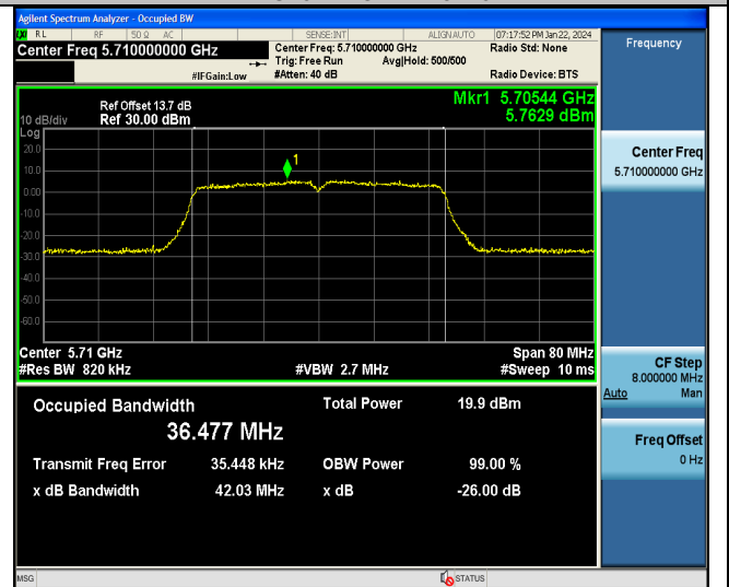
11AC40MIMO-Ant7-5710
