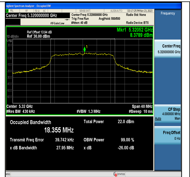
11AC20MIMO-Ant7-5320
