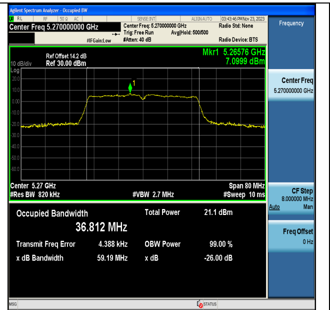
11AC40MIMO-Ant7-5270
