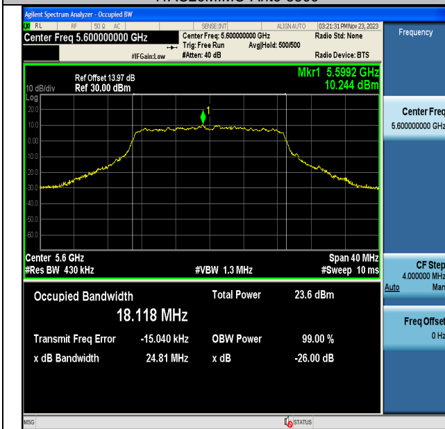
11AC20MIMO-Ant6-5600
