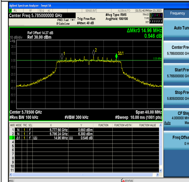
11N20MIMO-Ant6-5785-PASS
