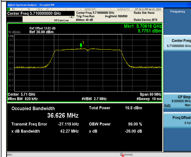
11AC40MIMO-Ant6-5710
