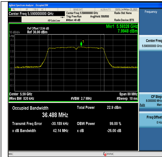
11AC40MIMO-Ant6-5590
