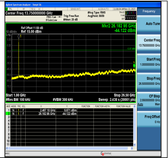
11N20MIMO-Ant7-2462-1000~26500-PASS
