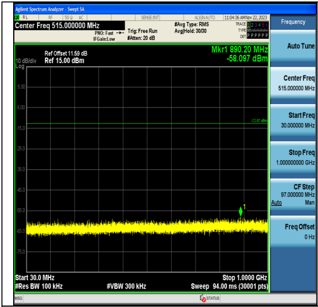
11N20MIMO-Ant7-2462-30~1000-PASS
