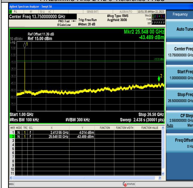
11N20MIMO-Ant6-2412-1000~26500-PASS
