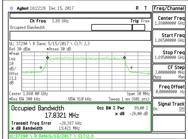
LTE B2 20MHz QPSK Middle Channel RB100-0
