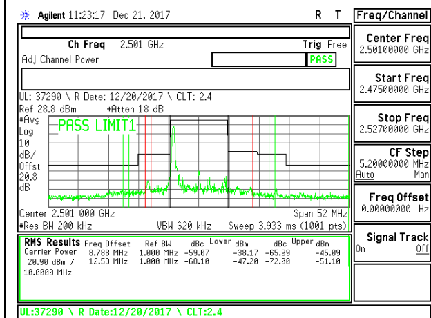
LTE B41 10MHz QPSK Low Channel RB1-0
