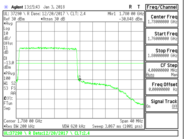
LTE B66 20MHz 16QAM High Channel RB50-0
