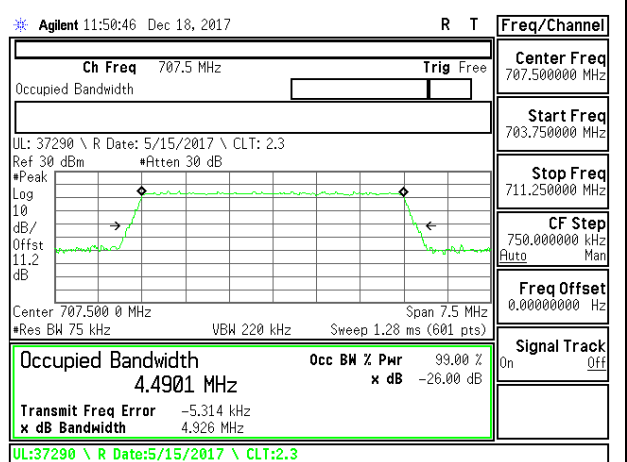
LTE B12 5MHz 16QAM Middle Channel RB25-0
