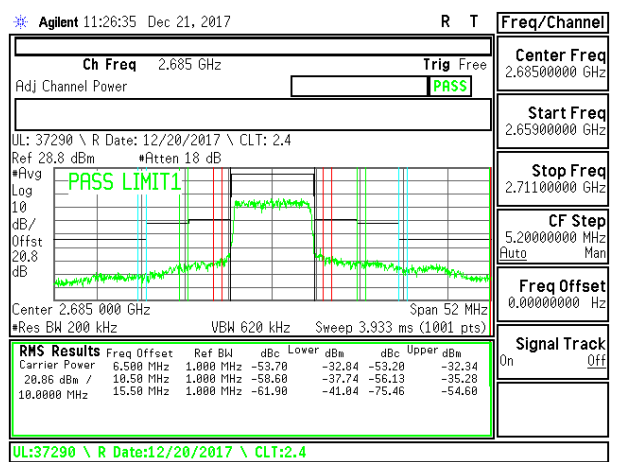
LTE B41 10MHz QPSK High Channel RB50-0
