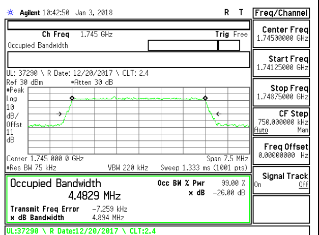
LTE B66 5MHz 16QAM Middle Channel RB25-0
