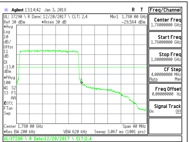
LTE B66 20MHz QPSK High Channel RB50-00
