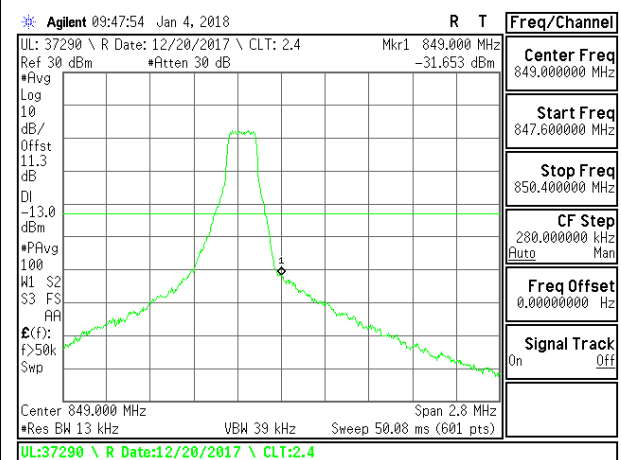
LTE B5 1.4MHz 16QAM High Channel RB1-5
