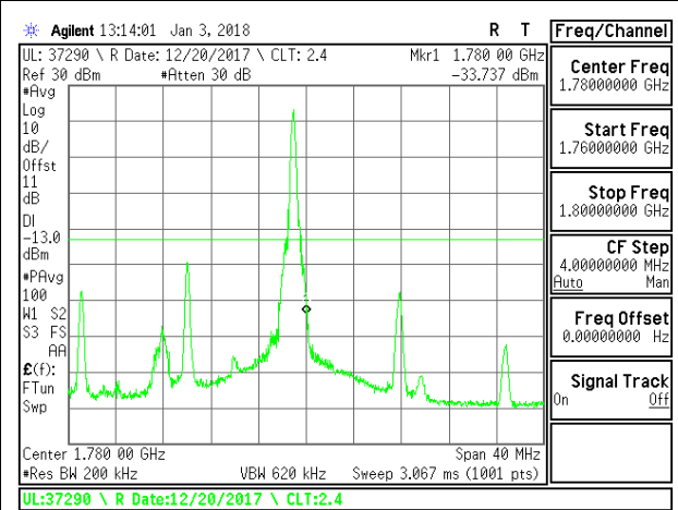
LTE B66 20MHz QPSK High Channel RB1-49
