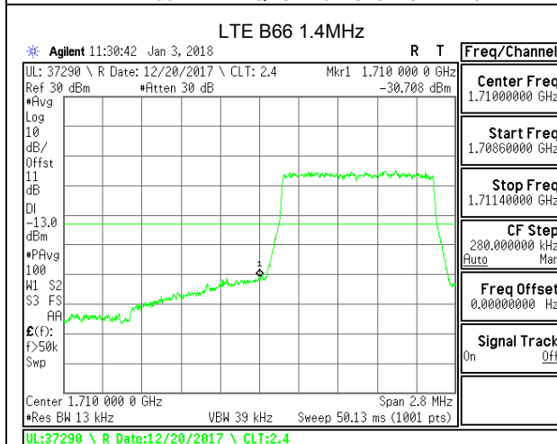
QPSK Low Channel RB6-0
