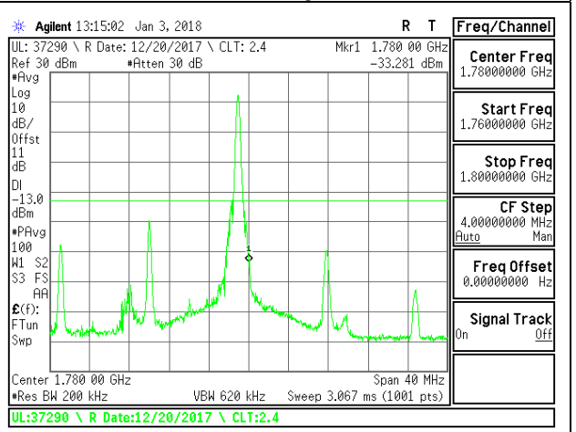
LTE B66 20MHz 16QAM High Channel RB1-49
