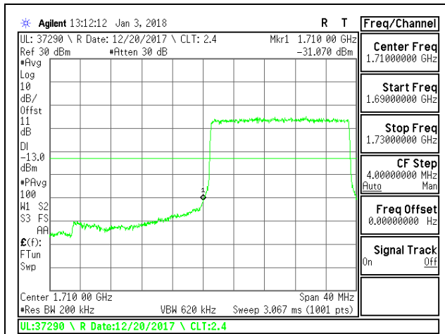
LTE B66 20MHz QPSK Low Channel RB50-0
