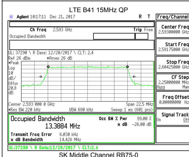
SK Middle Channel RB75-0
