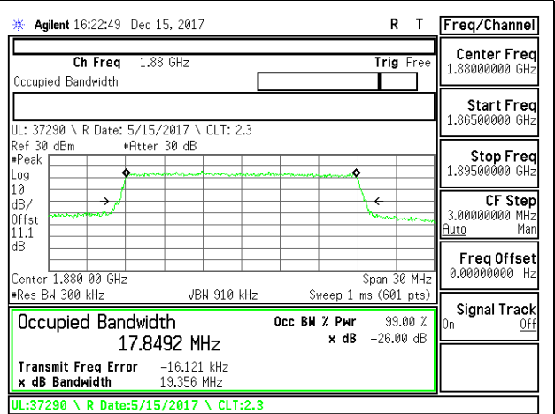
LTE B2 20MHz 16QAM Middle Channel RB100-0
