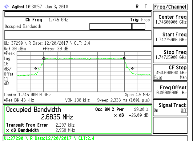
LTE B66 3MHz 16QAM Middle Channel RB15-0
