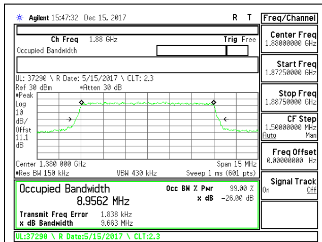
LTE B2 10MHz QPSK Middle Channel RB50-0
