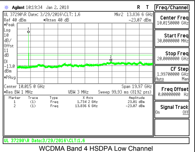
WCDMA Band 4 HSDPA Low Channel
