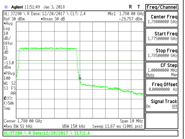
LTE B66 5MHz 16QAM High Channel RB25-0-0
