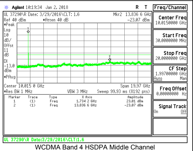
WCDMA Band 4 HSDPA Middle Channel
