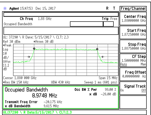
LTE B2 10MHz 16QAM Middle Channel RB50-0
