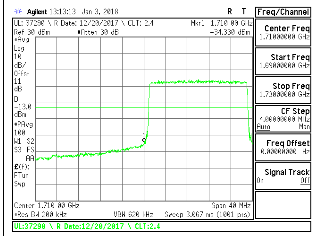
LTE B66 20MHz 16QAM Low Channel RB50-0
