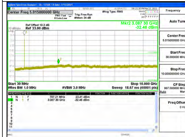
LTE17 10MHz QPSK HIGH Ch RB1-0
