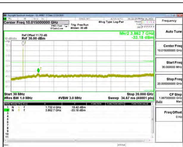
BAND 4 Rel 99 MID Channel
