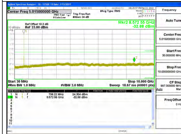
LTE17 10MHz 16QAM MID Ch RB1-0
