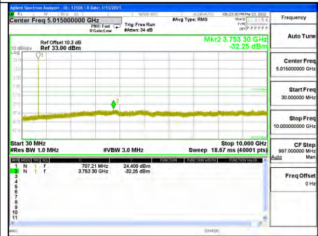
LTE17 10MHz 16QAM HIGH Ch RB1-0
