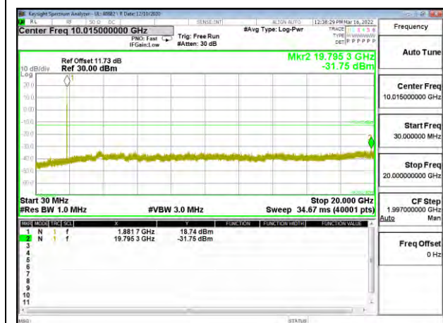
BAND 2 HSDPA MID Channel
