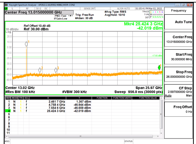
OUT-OF-BAND HIGH CHANNEL 10 CHAIN 0
