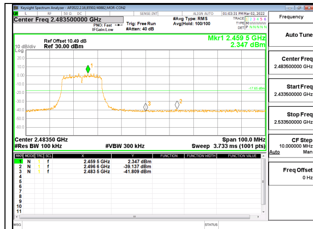
HIGH CHANNEL 10 BANDEDGE CHAIN 0
