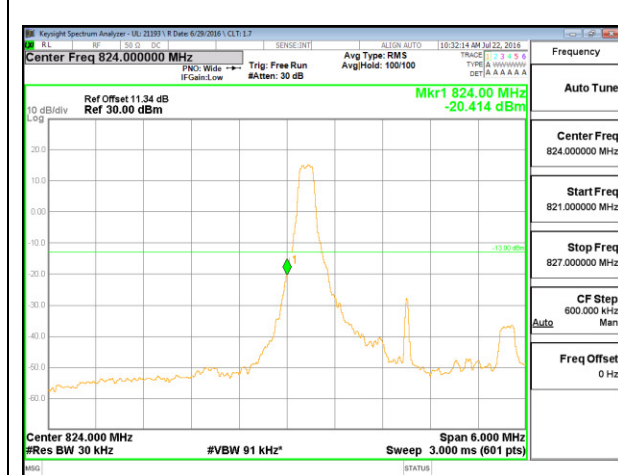
LTE B5 3MHz 16QAM Low Channel 1RB
