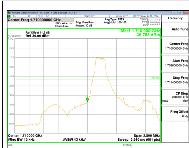
LTE B4 1.4MHz 16QAM Low Channel 1RB
