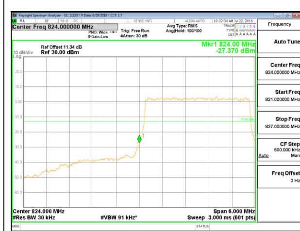
LTE B5 3MHz 16QAM Low Channel FRB
