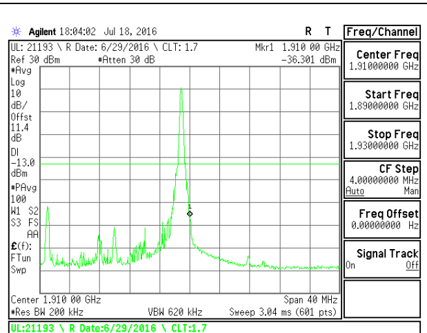
LTE B2 20MHz QPSK High Channel FRB
