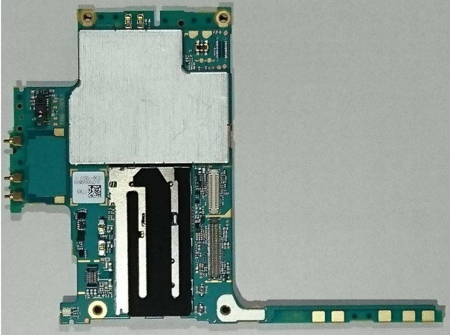
Internal PWB with Shield cases (Front-side)
