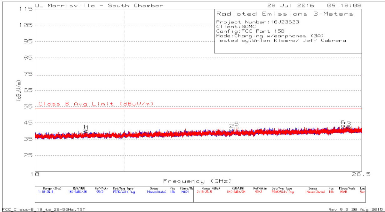
Figure 15 Radiated Emissions Graph – 18-26 GHz Charging
