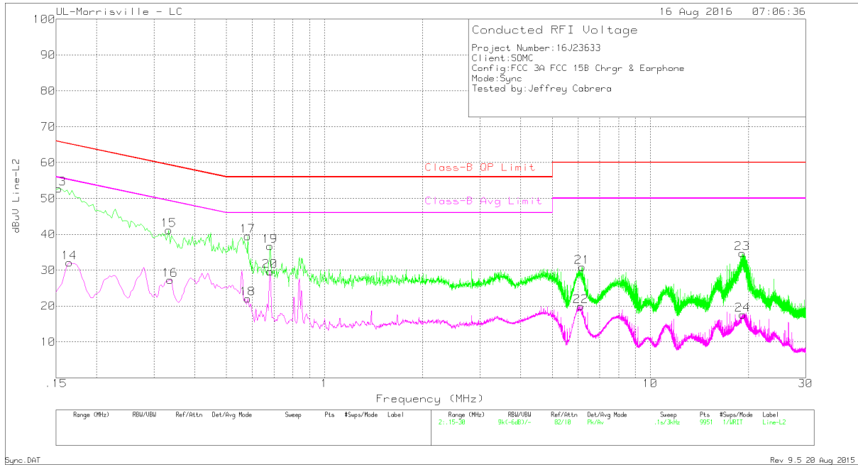
Figure 6 Conducted Emissions Graph – Line 2 Sync Mode (Laptop)
