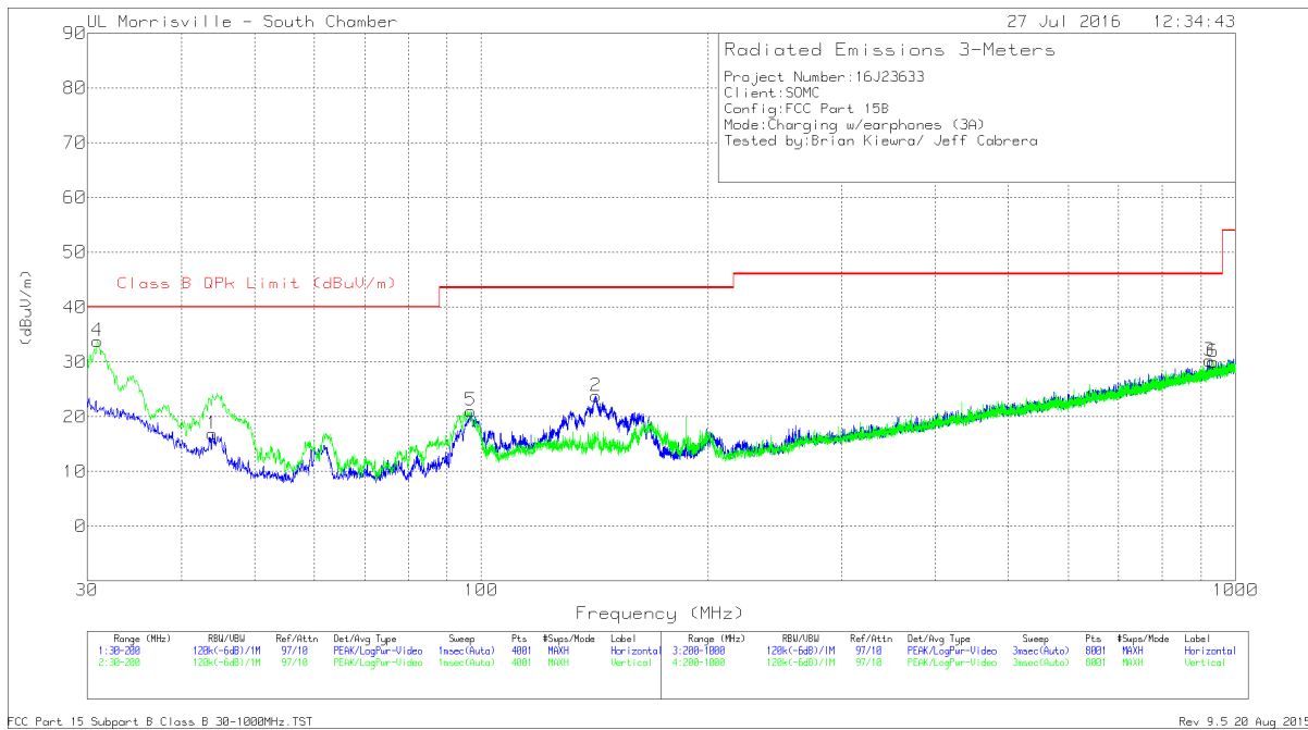
Figure 11 Radiated Emissions Graph – 30-1000 MHz Charging
