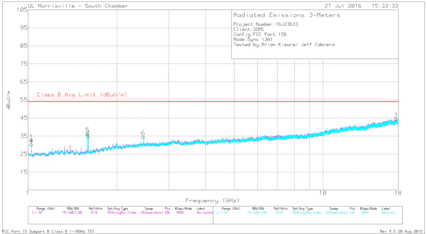
Figure 14 Radiated Emissions Graph – 1-18 GHz Sync
