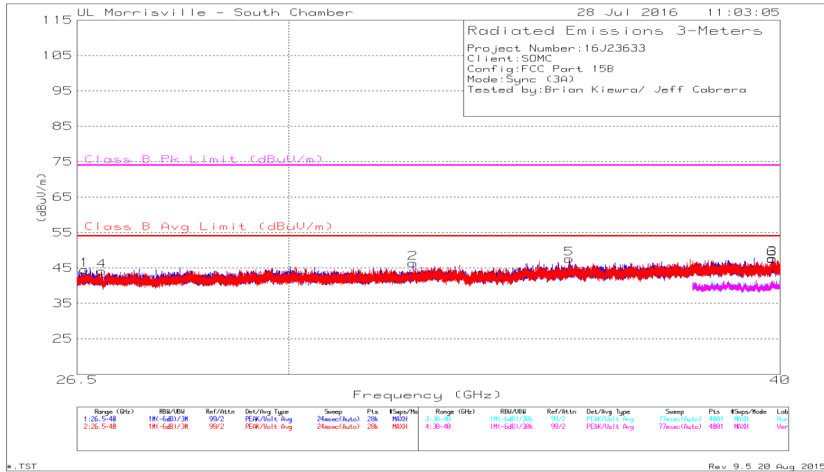
Figure 18 Radiated Emissions Graph – 26-40 GHz Sync
