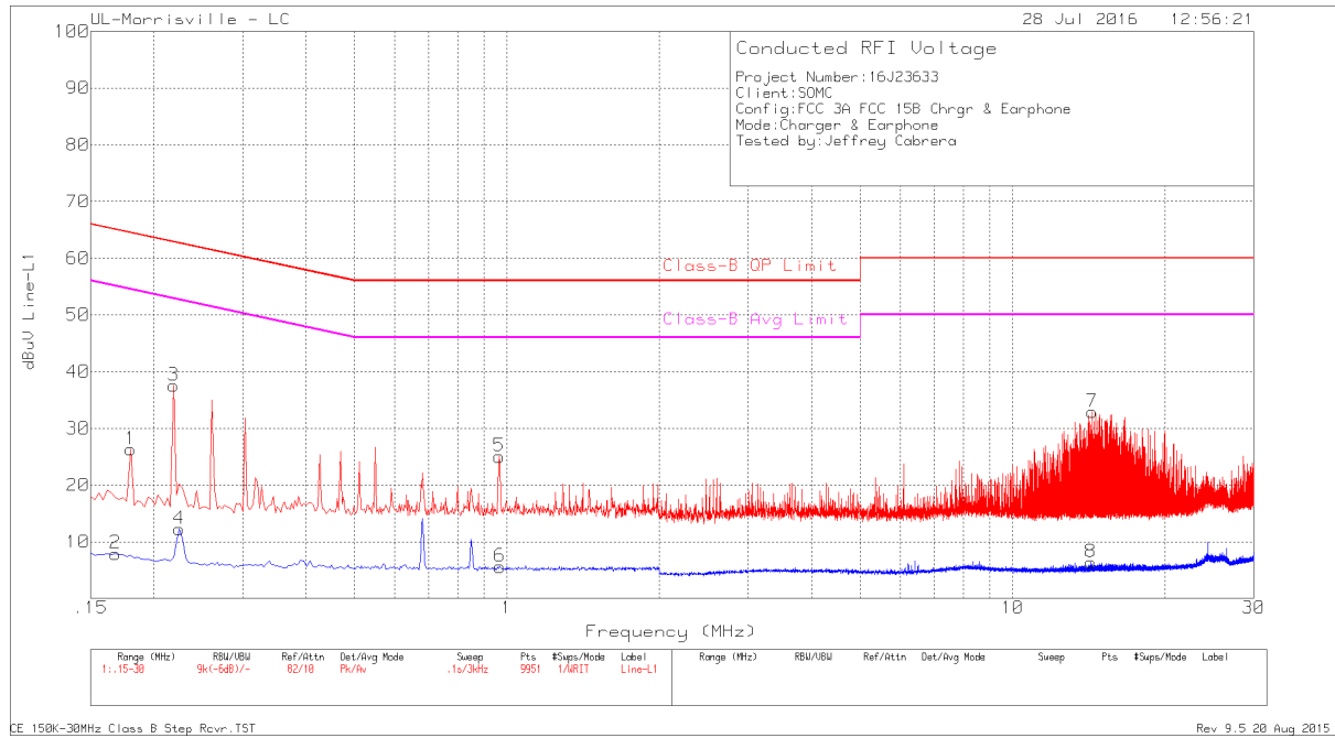
Figure 3 Conducted Emissions Graph – Line 1 Charging
