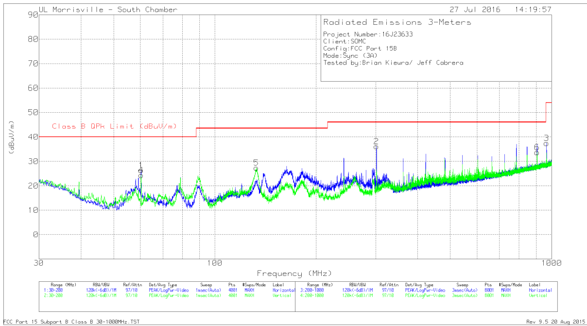
Figure 12 Radiated Emissions Graph – 30-1000 MHz Sync
