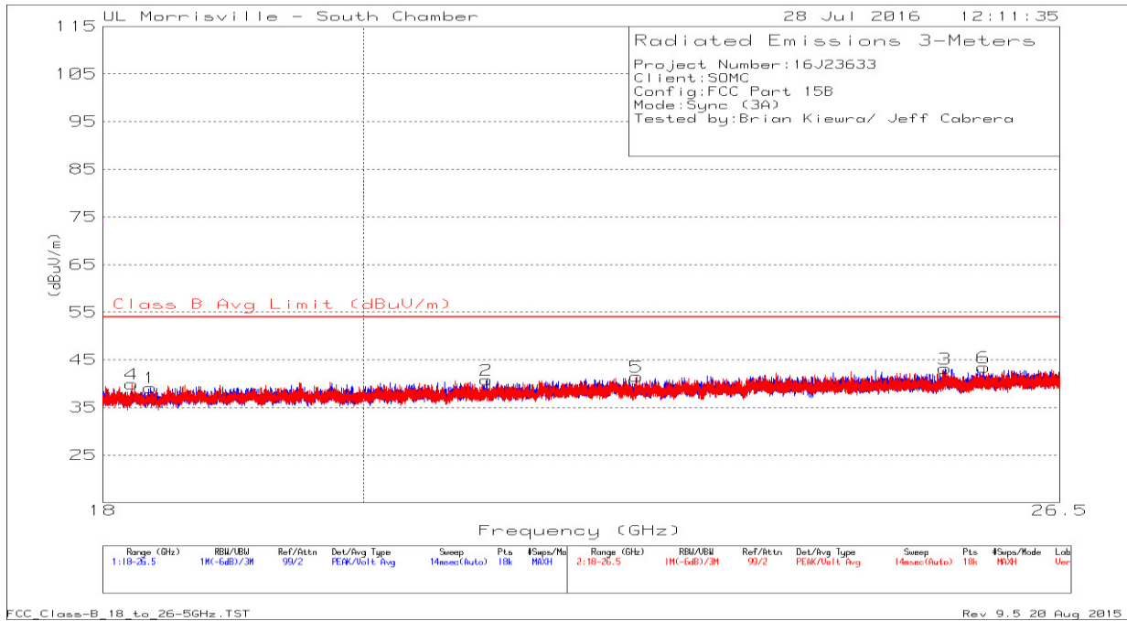
Figure 16 Radiated Emissions Graph – 18-26 GHz Sync
