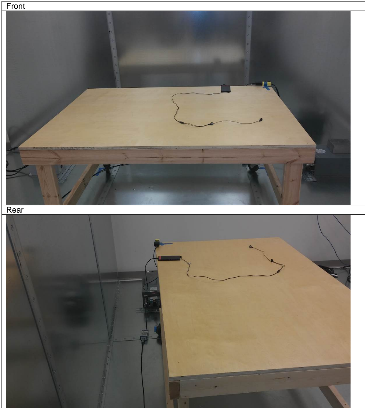
Figure 1 Test Setup for Conducted Emissions - Charger
