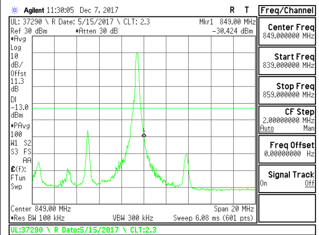
LTE B26 10MHz 16QAM High Channel RB1-49
