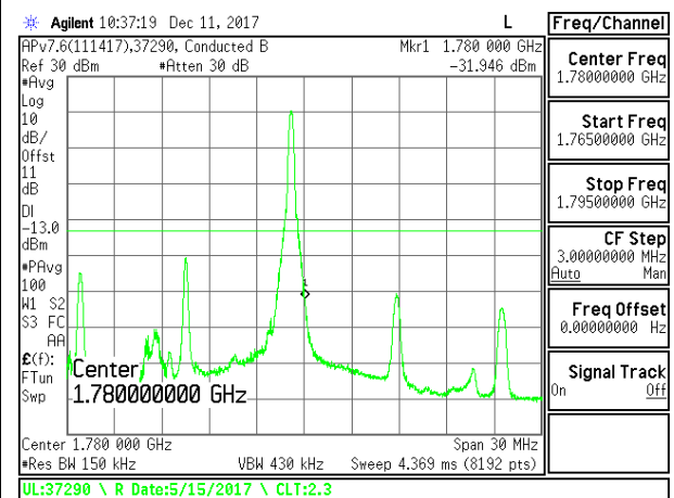
LTE B66 15MHz QPSK High Channel RB1-24
