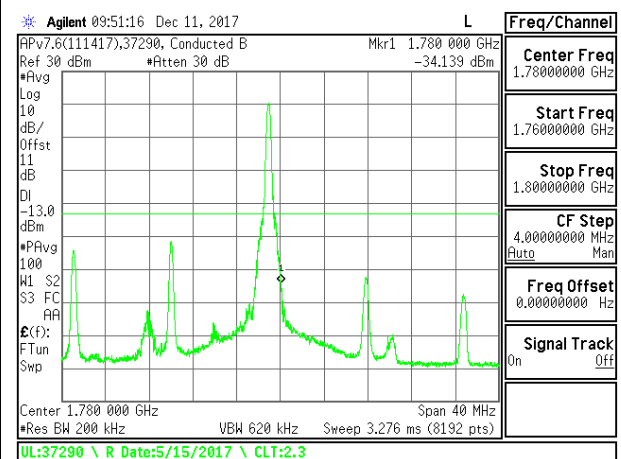
LTE B66 20MHz 16QAM High Channel RB1-49
