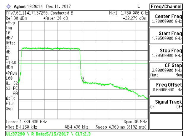
LTE B66 15MHz 16QAM High Channel RB25-0-0
