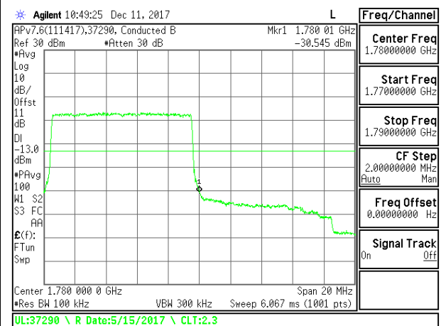
LTE B66 10MHz QPSK High Channel RB50-00
