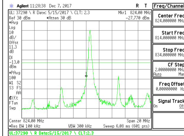
LTE B26 10MHz 16QAM Low Channel RB1-0
