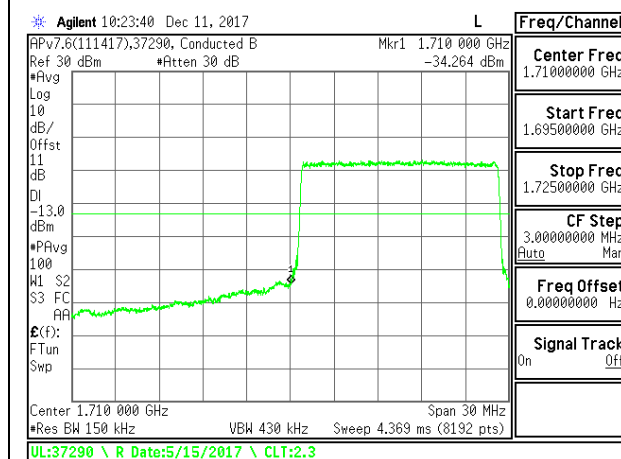
LTE B66 15MHz 16QAM Low Channel RB25-0
