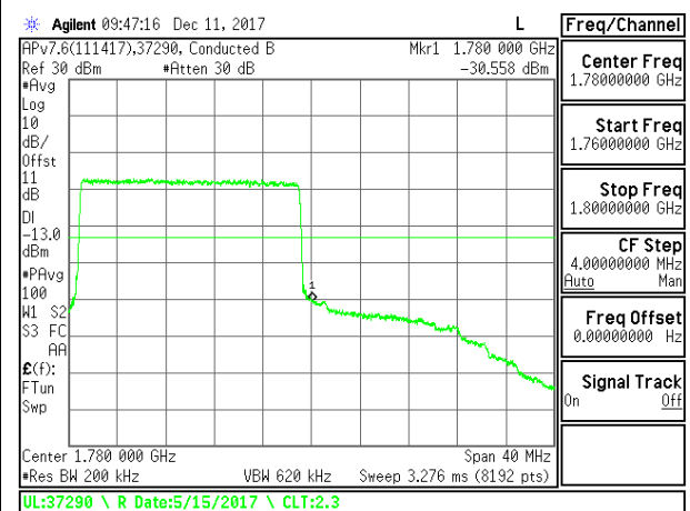
LTE B66 20MHz 16QAM High Channel RB50-0
