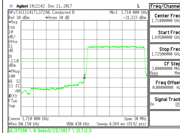
LTE B66 15MHz QPSK Low Channel RB25-0
