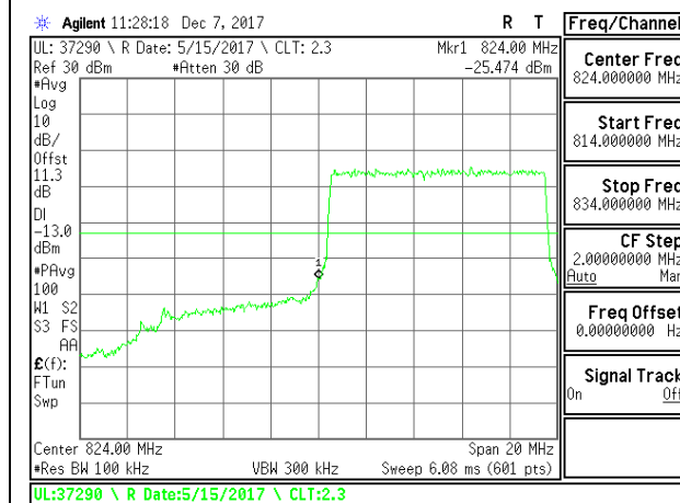
LTE B26 10MHz QPSK Low Channel RB50-0
