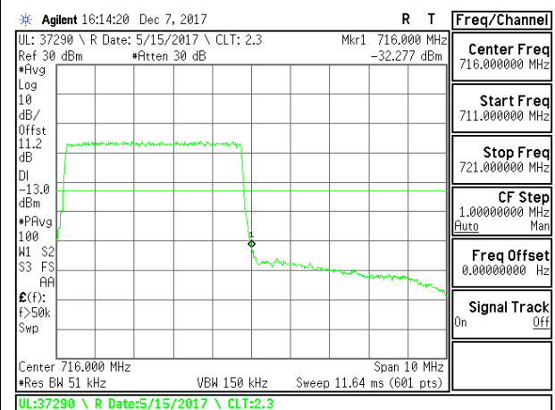
LTE B12 5MHz 16QAM High Channel RB25-0
