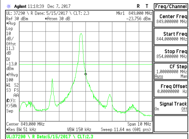
LTE B26 5MHz 16QAM High Channel RB1-24
