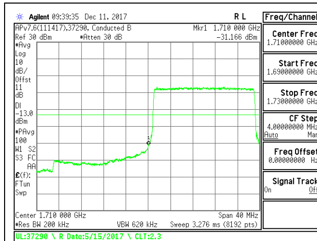
LTE B66 20MHz QPSK Low Channel RB50-0
