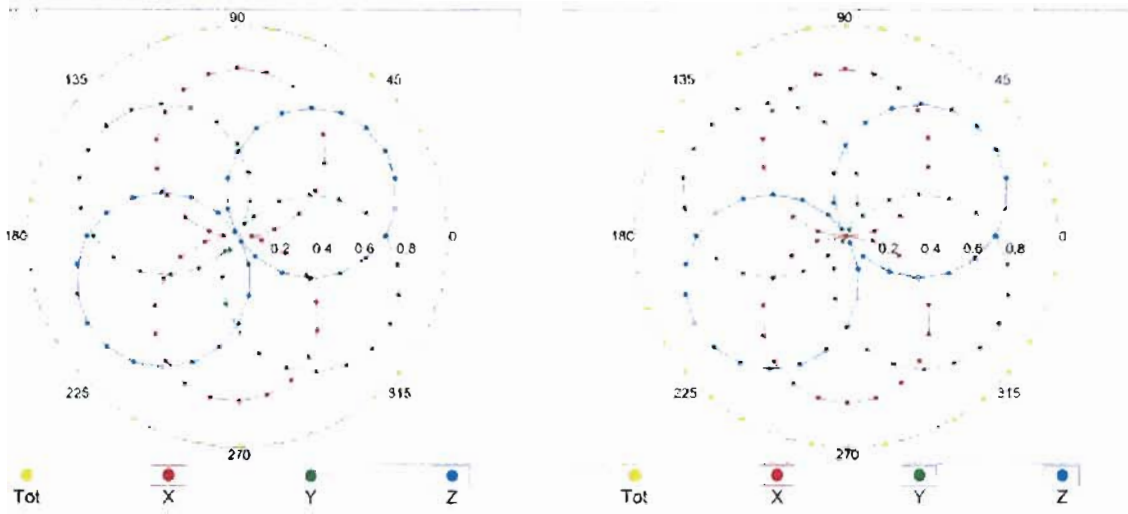
f=600 MHz,TEM
