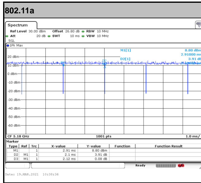
MIMO <Chain 0>
