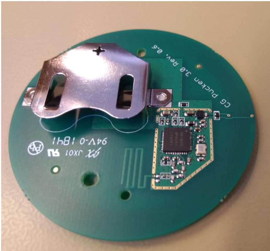
Fig.6 PCB back view
