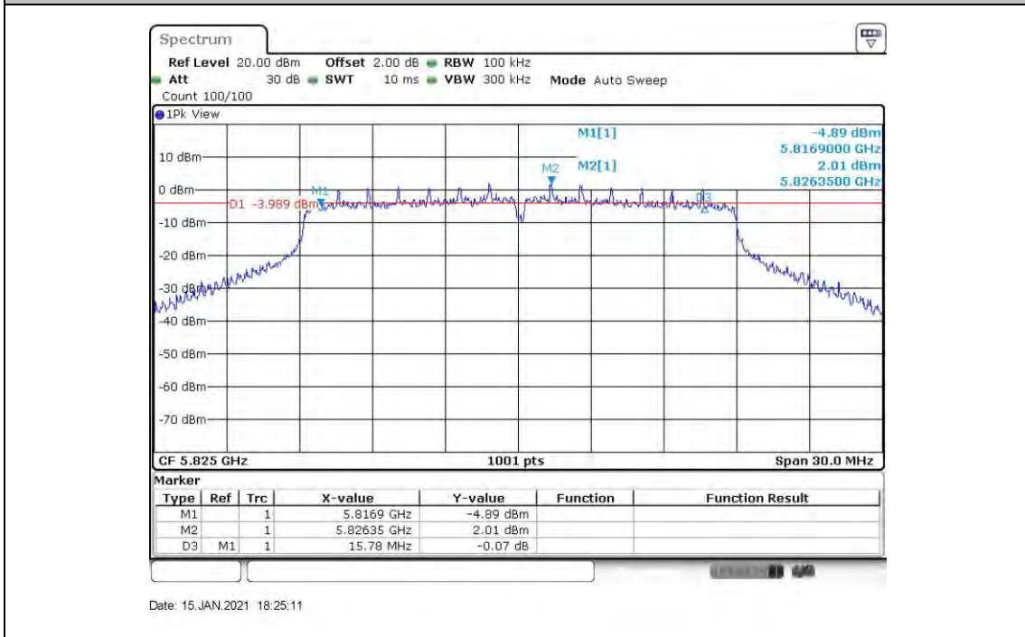
11AC20SISO_ANT7_5825
