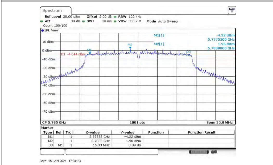
11A_ANT6_5785
