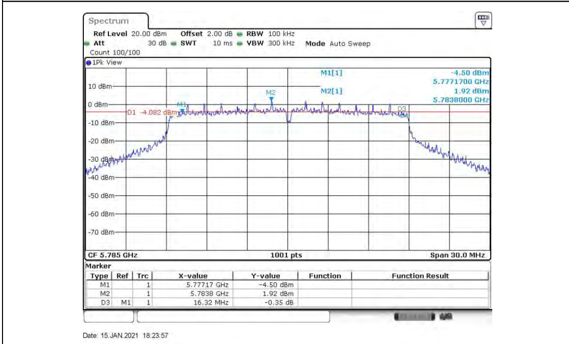
11AC20SISO_ANT6_5785
