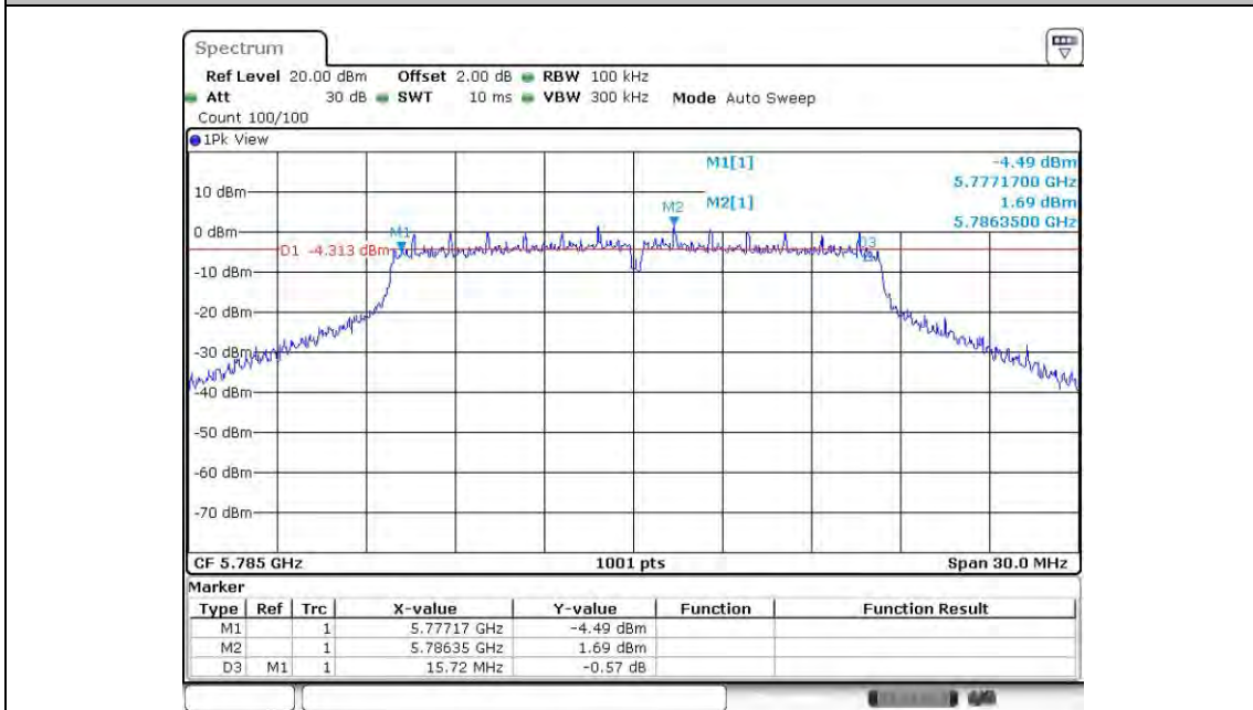
11A-CDD_ANT6_5785
