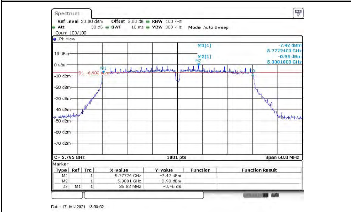
11AC40SISO_ANT6_5795
