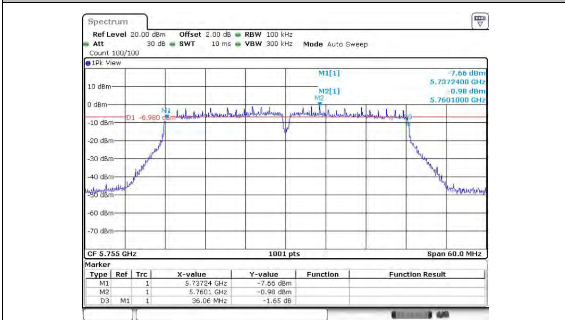
11N40SISO_ANT6_5755
