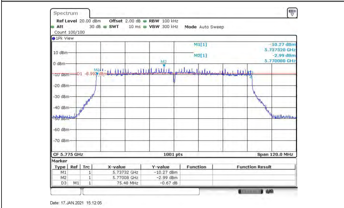
11AC80SISO_ANT6_5775
