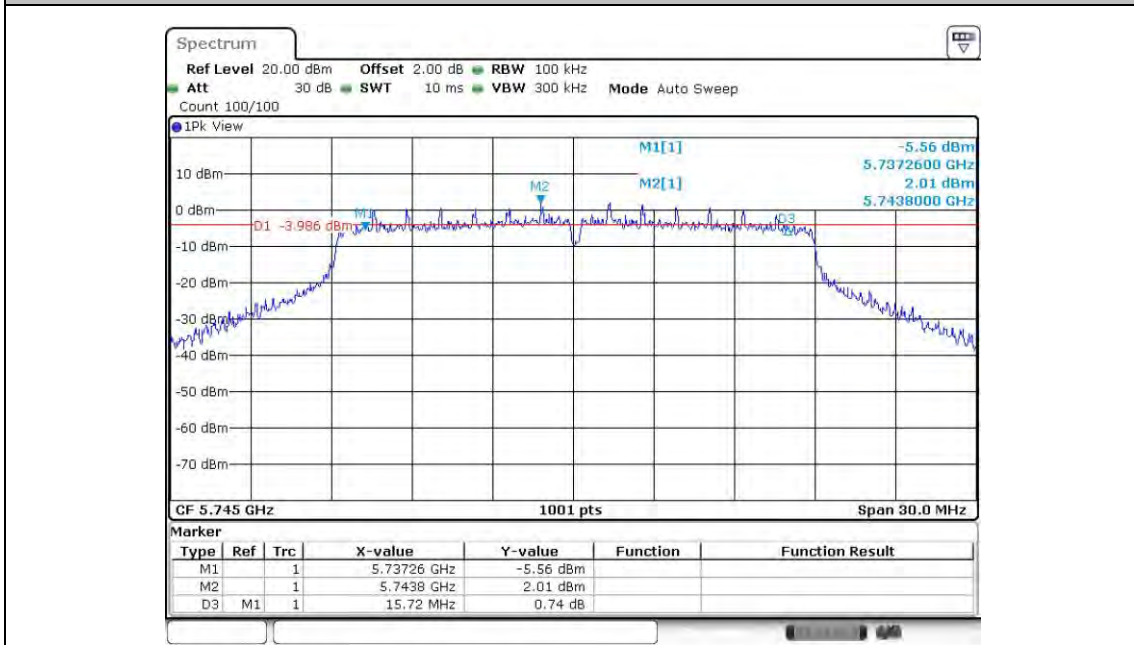
11N20SISO_ANT6_5745
