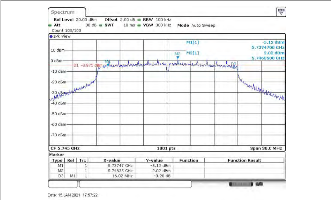
11AC20SISO_ANT6_5745
