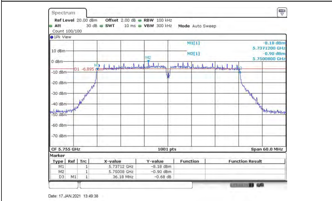
11AC40SISO_ANT6_5755
