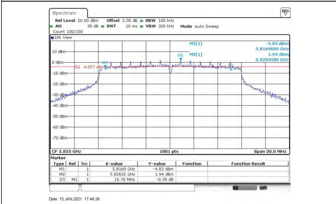
11N20SISO_ANT6_5825
