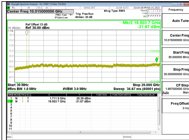
LTE66 10MHz QPSK LOW Ch RB1-0
