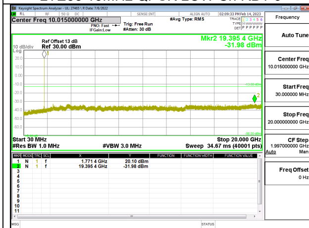
LTE66 10MHz QPSK HIGH Ch RB1-0
