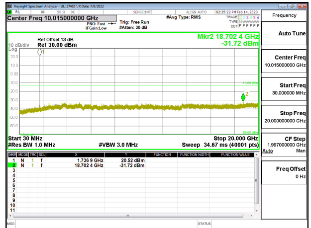
LTE66 20MHz QPSK MID Ch RB1-0
