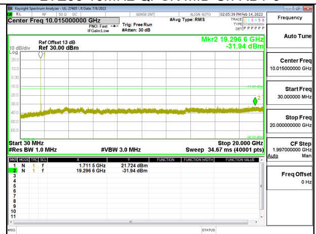
LTE66 10MHz 16QAM LOW Ch RB1-0
