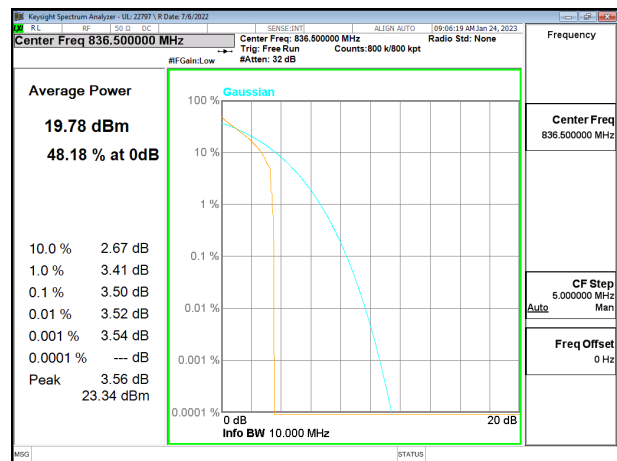
LTE5 3MHz 16QAM MID Ch
