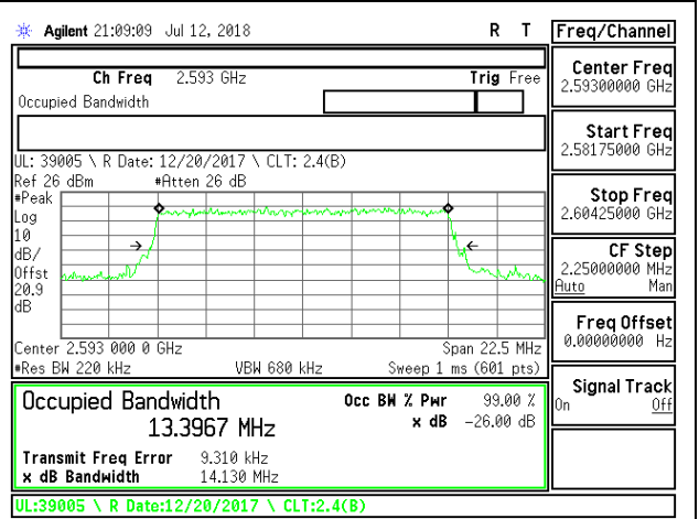
LTE B41 15MHz 16QAM Mid Channel RB75-0
