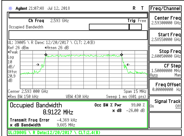
LTE B41 10MHz QPSK Mid Channel RB50-0
