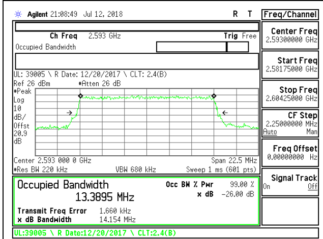
LTE B41 15MHz QPSK Mid Channel RB75-0
