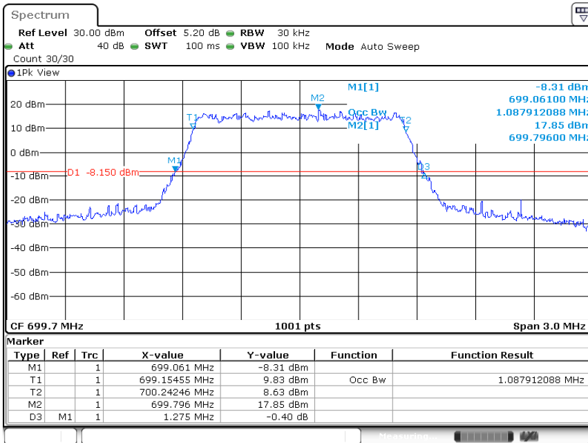
Band12-1.4MHz-QPSK-23017-6RB#0-1.088
