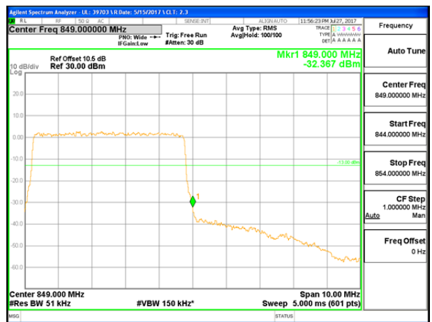
LTE B5 5MHz 16QAM High Channel FRB
