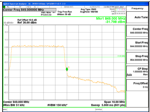
LTE B5 5MHz QPSK High Channel FRB
