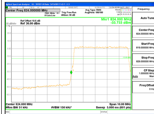
LTE B5 5MHz 16QAM Low Channel FRB
