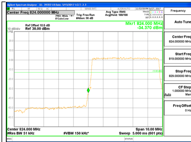
LTE B5 5MHz QPSK Low Channel FRB
