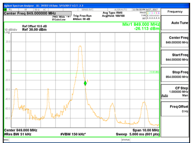
LTE B5 5MHz 16QAM High Channel 1RB
