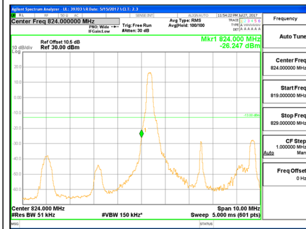
LTE B5 5MHz 16QAM Low Channel 1RB
