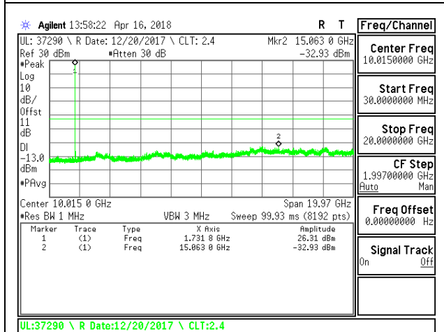
LTE B4 1.4MHz QPSK Middle Channel RB1-0
