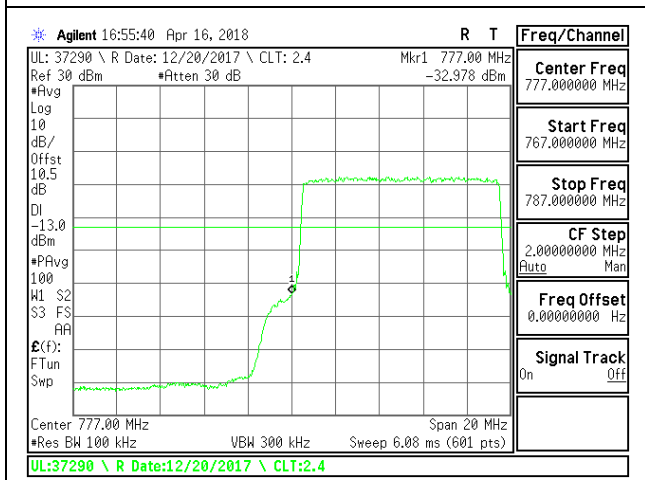
LTE B13 10MHz 16QAM Low Channel RB50-0
