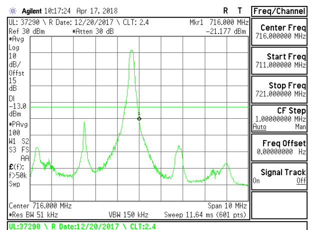
LTE B17 5MHz 16QAM High Channel RB1-0
