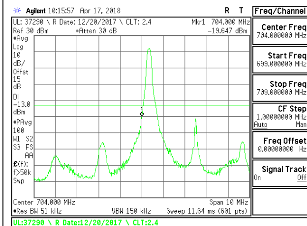
LTE B17 5MHz 16QAM Low Channel RB1-0
