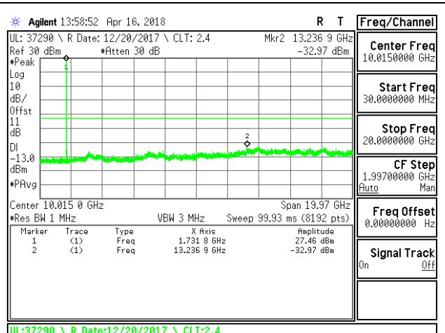
LTE B4 1.4MHz 16QAM Middle Channel RB1-0
