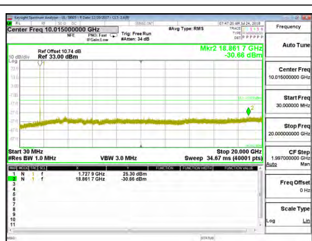
LTE B4 10MHz QPSK Mid Channel RB1-0
