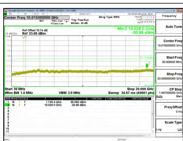
LTE B4 10MHz 16QAM High Channel RB1-0
