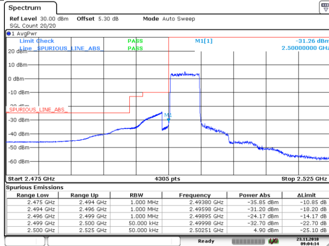
Band7_5MHz_QPSK_20775_25RB#0
