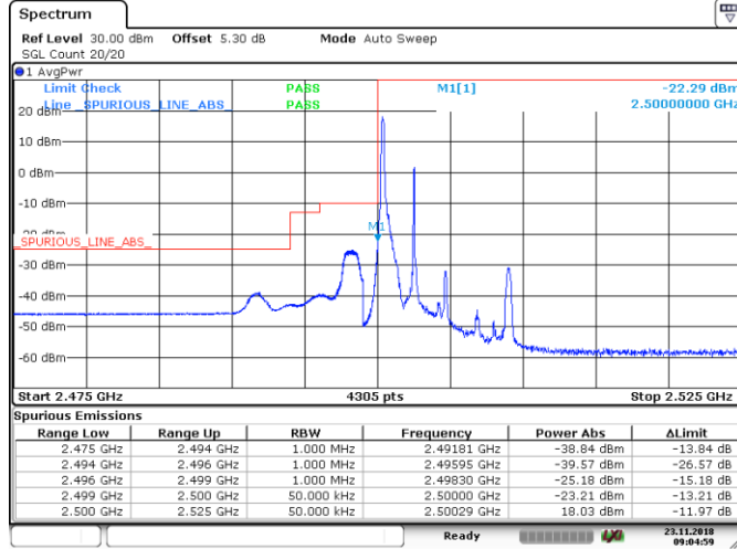
Band7_5MHz_QPSK_20775_1RB#0
