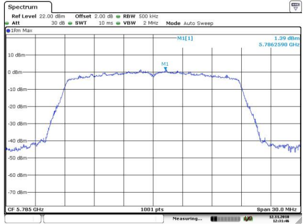
Power Spectral Density Data Plot (CH Mid 5785 MHz)
