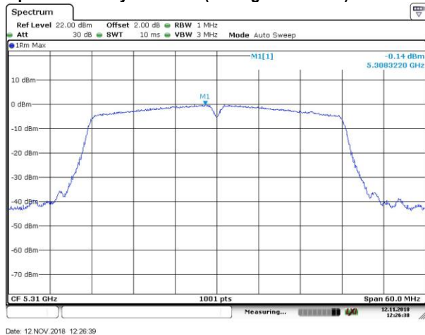
Power Spectral Density Data Plot (CH High 5310 MHz)
