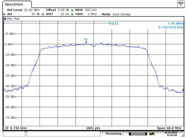
802.11n HT20, 5725~5850 MHz Power Spectral Density Data Plot (CH Low 5745 MHz)
