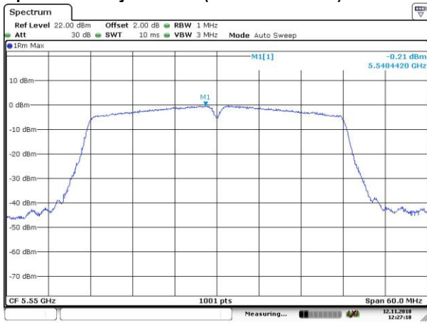
Power Spectral Density Data Plot (CH Mid 5550 MHz)
