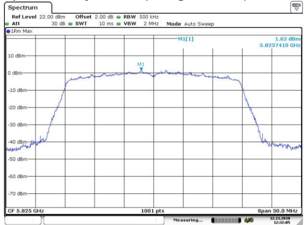
Power Spectral Density Data Plot (CH High 5825 MHz)
