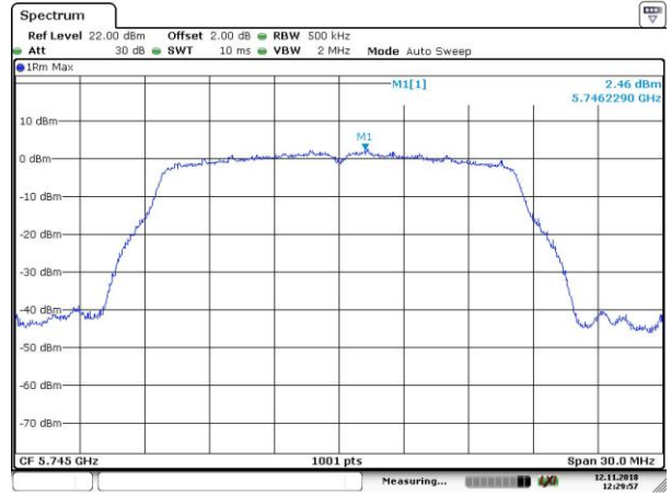
802.11a 5725~5850 MHz Power Spectral Density Data Plot (CH Low 5745 MHz)
