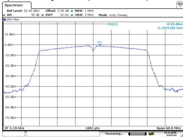
802.11n HT40, 5150~5250 MHz Power Spectral Density Data Plot (CH Low 5190 MHz)
