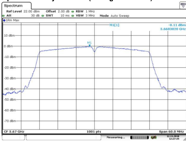
Power Spectral Density Data Plot (CH High 5670 MHz)
