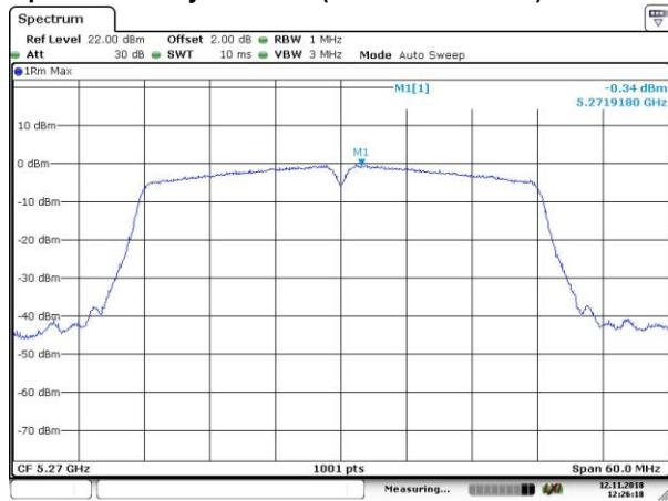
802.11n HT40, 5250~5350 MHz Power Spectral Density Data Plot (CH Low 5270 MHz)
