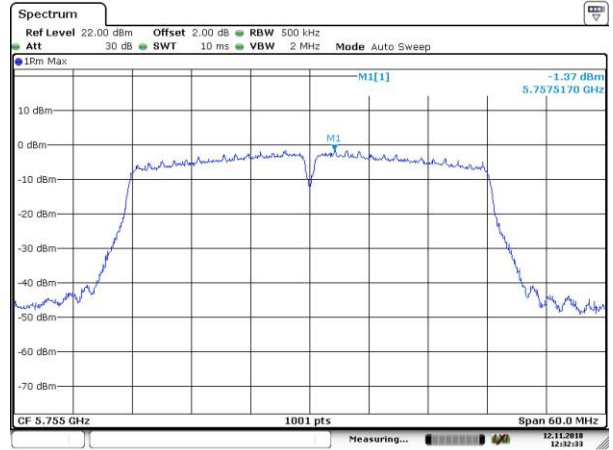
802.11n HT40, 5725~5850 MHz Power Spectral Density Data Plot (CH Low 5755 MHz)
