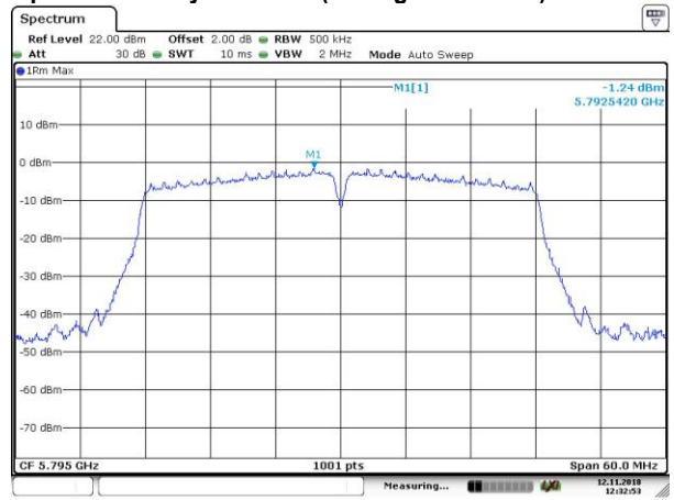
Power Spectral Density Data Plot (CH High 5795 MHz)
