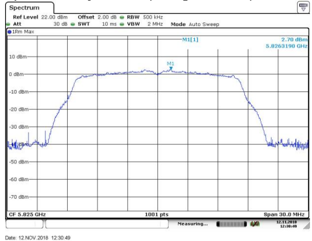
Power Spectral Density Data Plot (CH High 5825 MHz)
