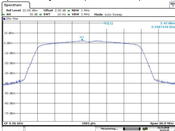
802.11n HT20, 5250~5350 MHz Power Spectral Density Data Plot (CH Low 5260MHz)
