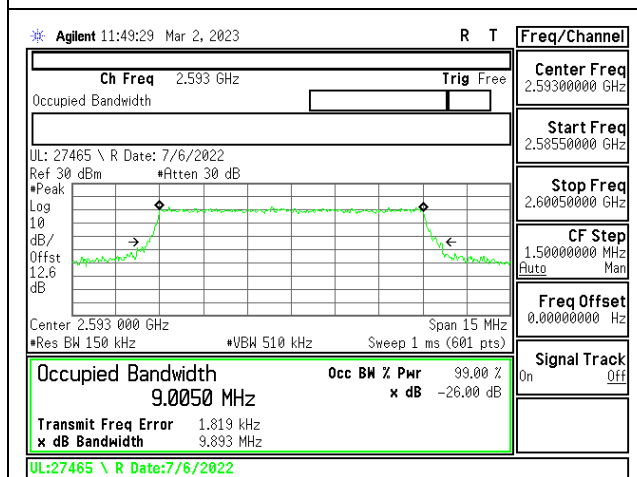
LTE41 10MHz QPSK MID Ch RB50-0
