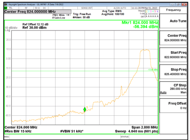
LTE5 1.4MHz 16QAM LOW Ch RB1-5
