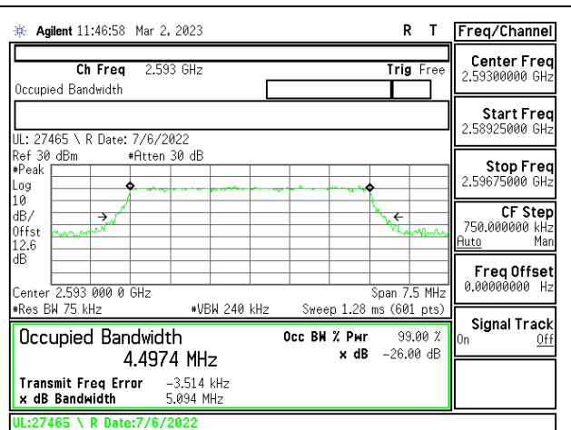
LTE41 5MHz 16QAM MID Ch RB25-0
