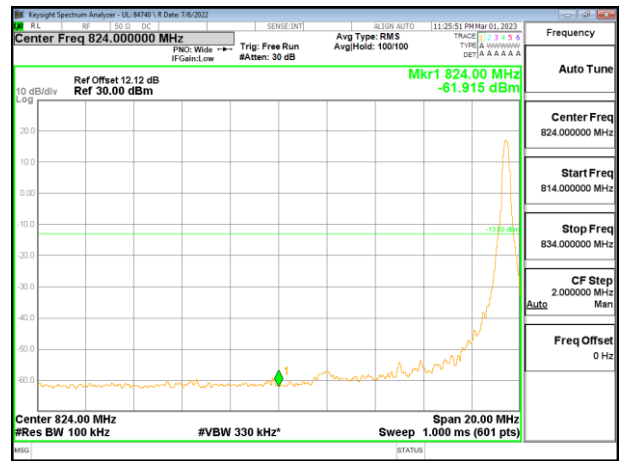
LTE5 10MHz QPSK LOW Ch RB1-49
