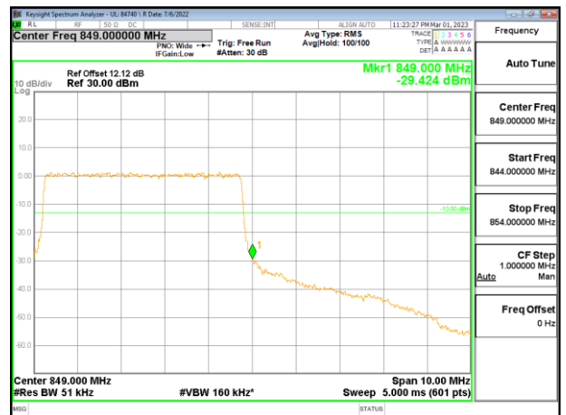
LTE5 5MHz QPSK HIGH Ch RB25-0
