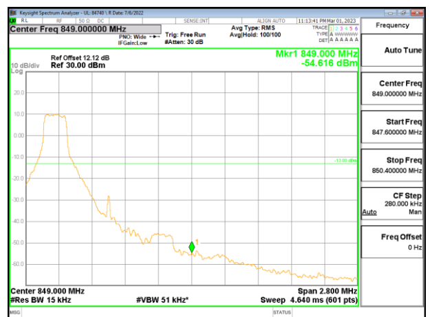
LTE5 1.4MHz 16QAM HIGH Ch RB1-0
