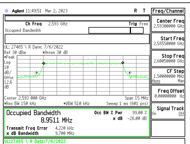
LTE41 10MHz 16QAM MID Ch RB50-0
