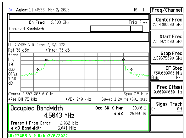
LTE41 5MHz QPSK MID Ch RB25-0
