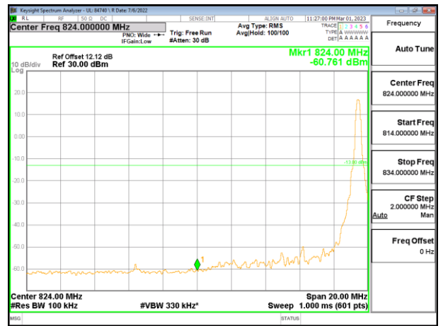
LTE5 10MHz 16QAM LOW Ch RB1-49
