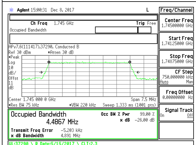
LTE B66 5MHz QPSK Middle Channel RB25-0
