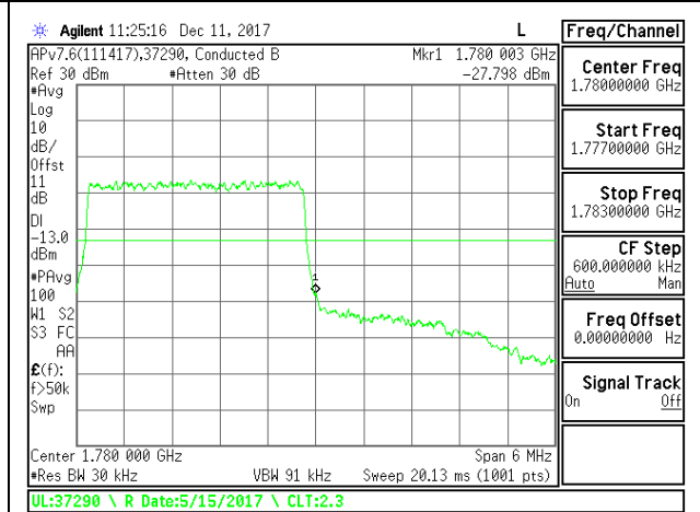
LTE B66 3MHz 16QAM High Channel RB1-14
