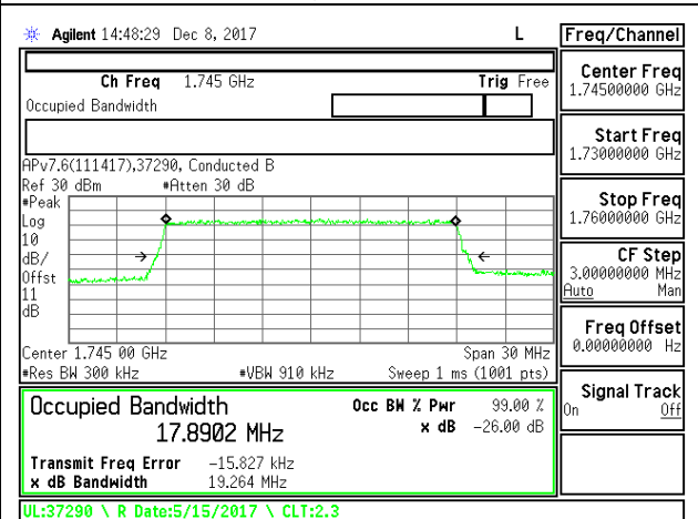
LTE B66 20MHz 16QAM Middle Channel RB100-0
