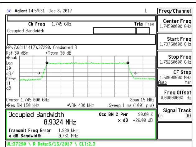
LTE B66 10MHz 16QAM Middle Channel RB50-0
