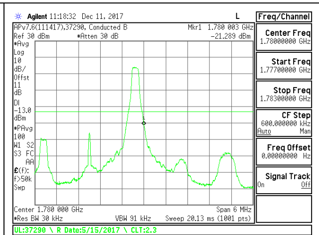
LTE B66 3MHz 16QAM High Channel RB1-49
