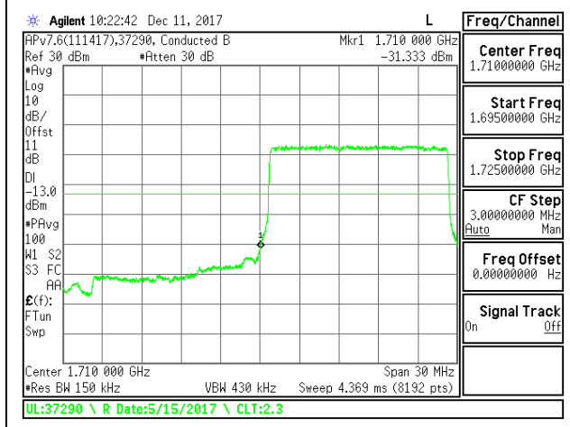
LTE B66 15MHz QPSK Low Channel RB25-0
