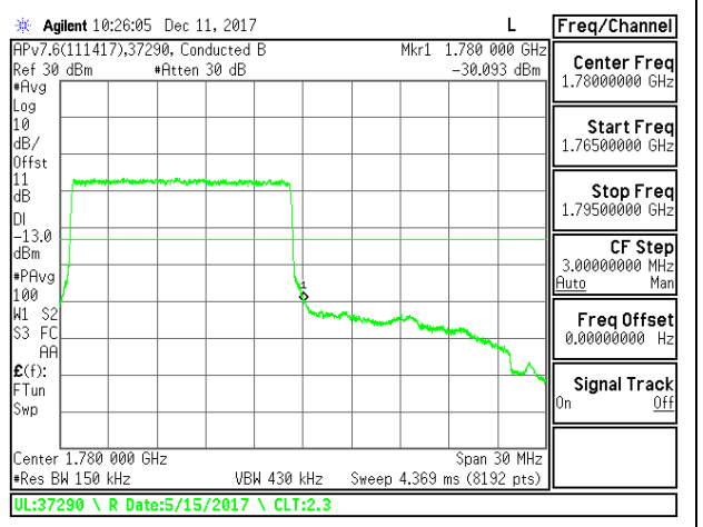
LTE B66 15MHz QPSK High Channel RB25-0
