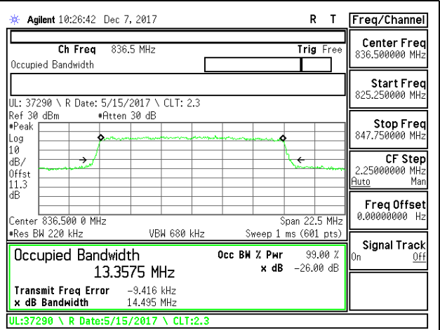
LTE B26 15MHz 16QAM Middle Channel RB75-0
