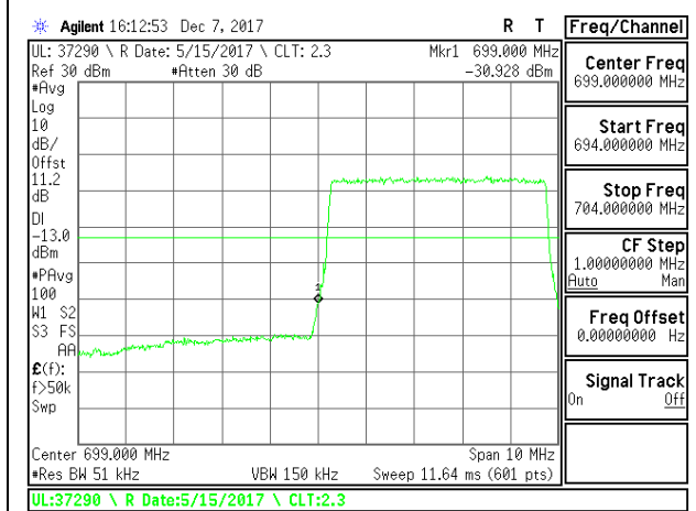
LTE B12 5MHz 16QAM Low Channel RB25-0
