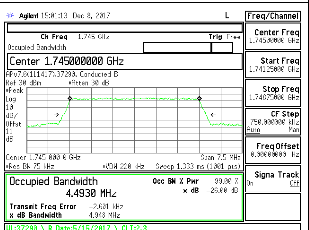
LTE B66 5MHz 16QAM Middle Channel RB25-0
