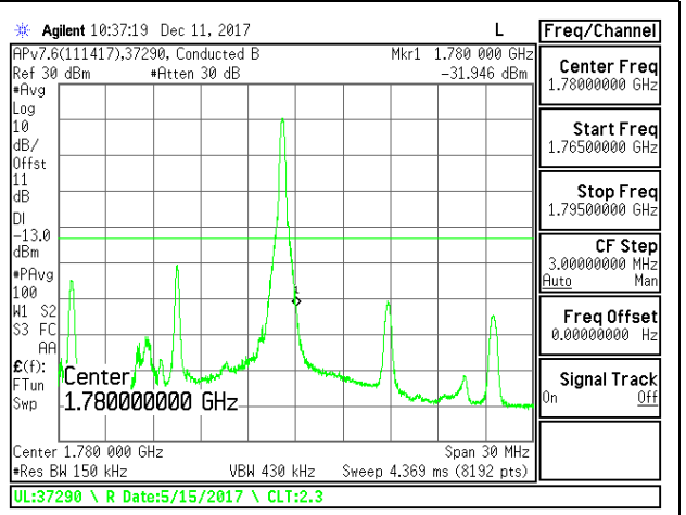
LTE B66 15MHz QPSK High Channel RB1-24
