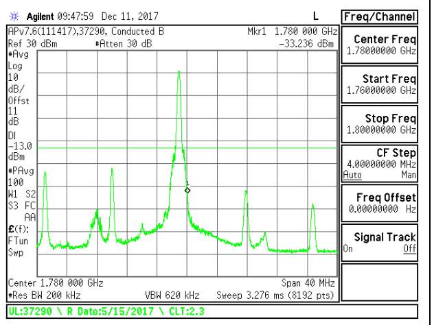
LTE B66 20MHz QPSK High Channel RB1-49
