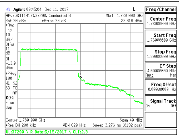
LTE B66 20MHz QPSK High Channel RB50-00
