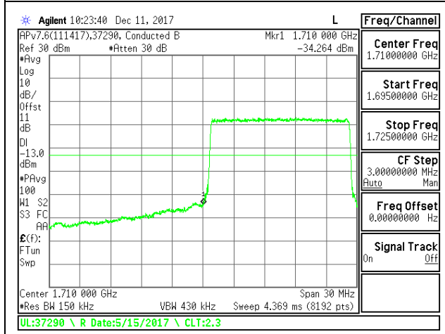
LTE B66 15MHz 16QAM Low Channel RB25-0
