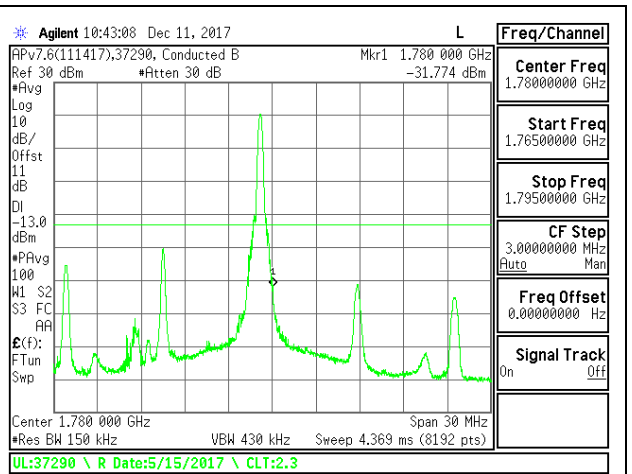
LTE B66 15MHz 16QAM High Channel RB1-24
