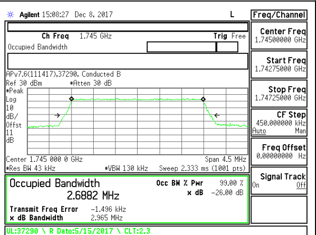
LTE B66 3MHz 16QAM Middle Channel RB15-0
