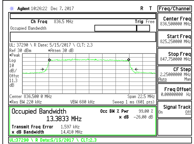
LTE B26 15MHz QPSK Middle Channel RB75-0
