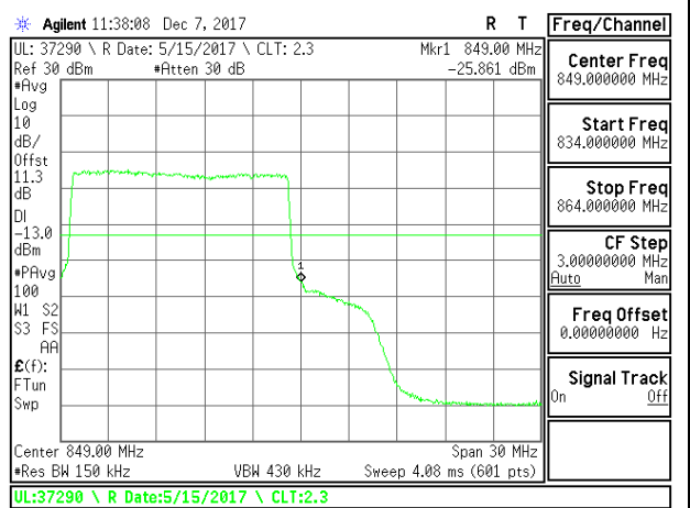
LTE B26 15MHz QPSK High Channel RB75-0
