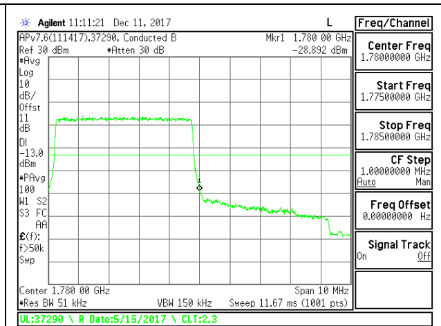
LTE B66 5MHz QPSK High Channel RB25-0
