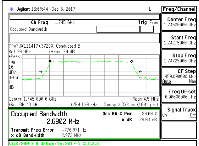
LTE B66 3MHz QPSK Middle Channel RB15-0
