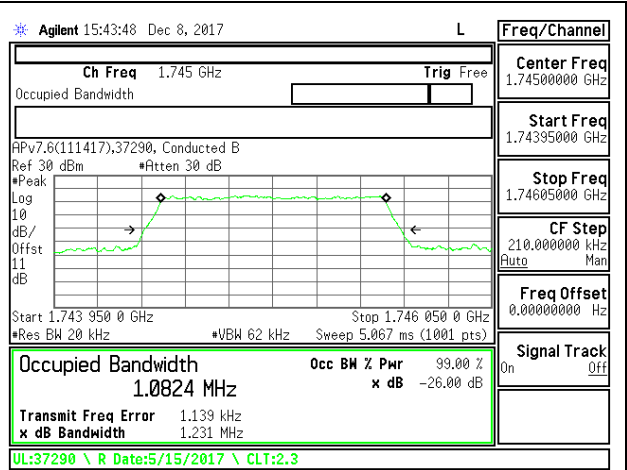
LTE B66 1.4MHz 16QAM Middle Channel RB6-0
