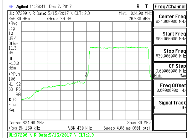
LTE B26 15MHz QPSK Low Channel RB75-0
