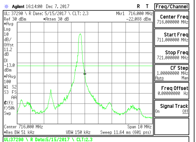
LTE B12 5MHz 16QAM High Channel RB1-24
