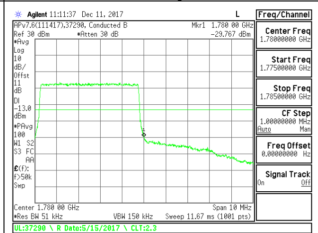
LTE B66 5MHz 16QAM High Channel RB25-0-0
