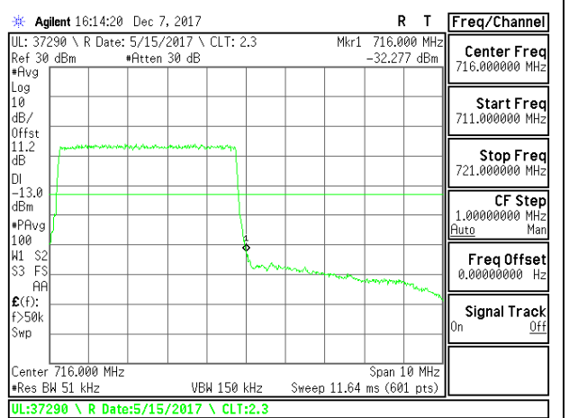
LTE B12 5MHz 16QAM High Channel RB25-0
