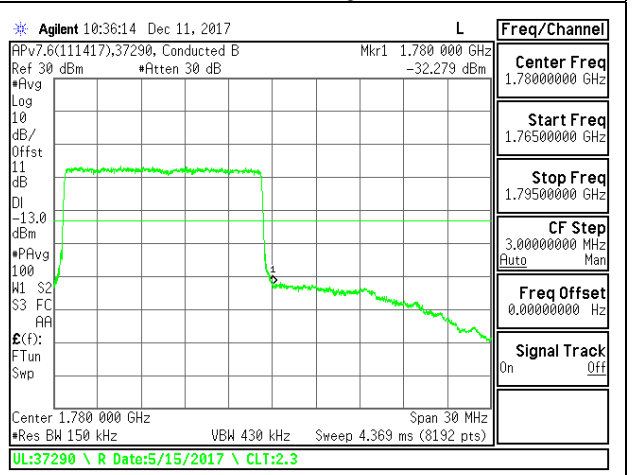
LTE B66 15MHz 16QAM High Channel RB25-0-0
