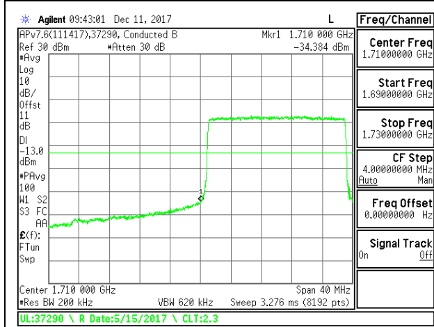
LTE B66 20MHz 16QAM Low Channel RB50-0
