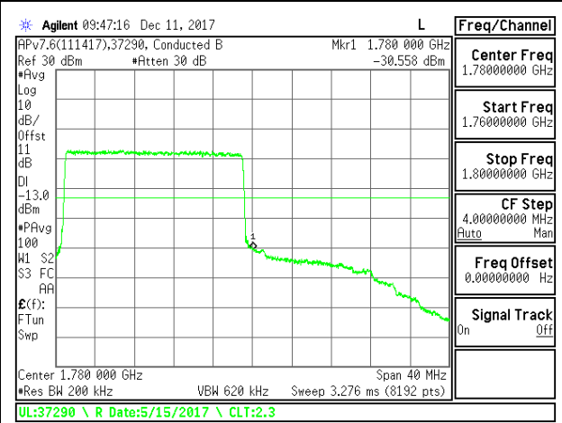
LTE B66 20MHz 16QAM High Channel RB50-0
