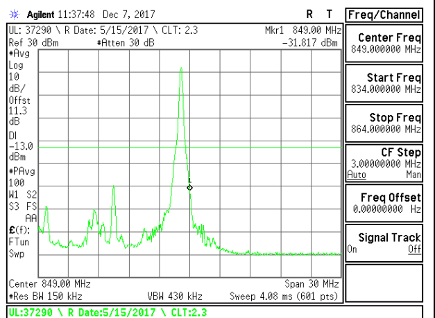
LTE B26 15MHz QPSK High Channel RB1-74
