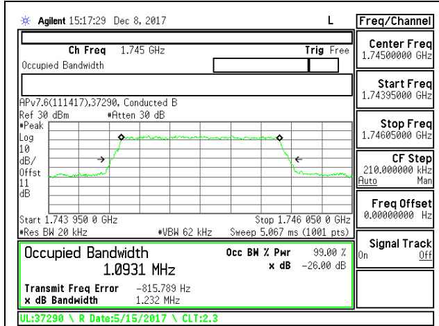
LTE B66 1.4MHz QPSK Middle Channel RB6-0
