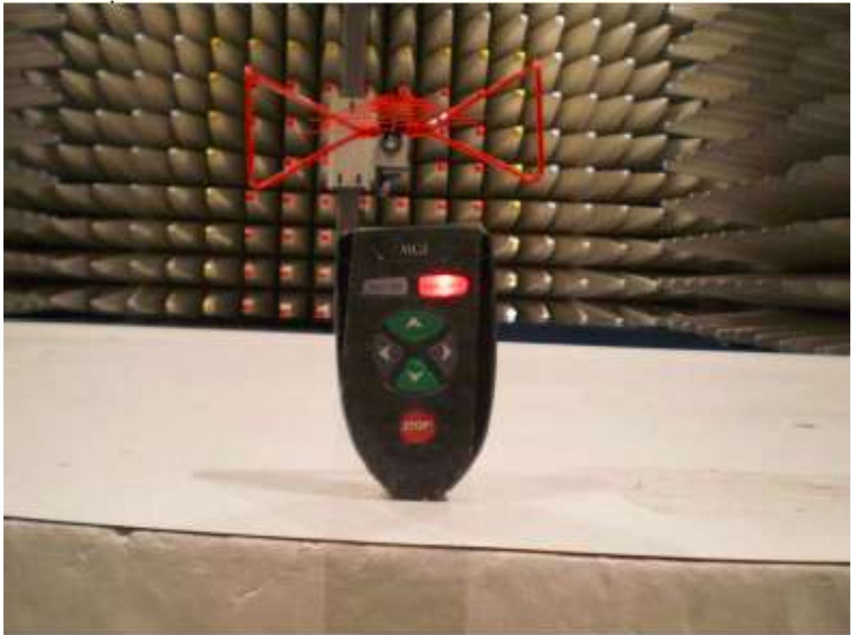
NavRemote Test Setup Photos
