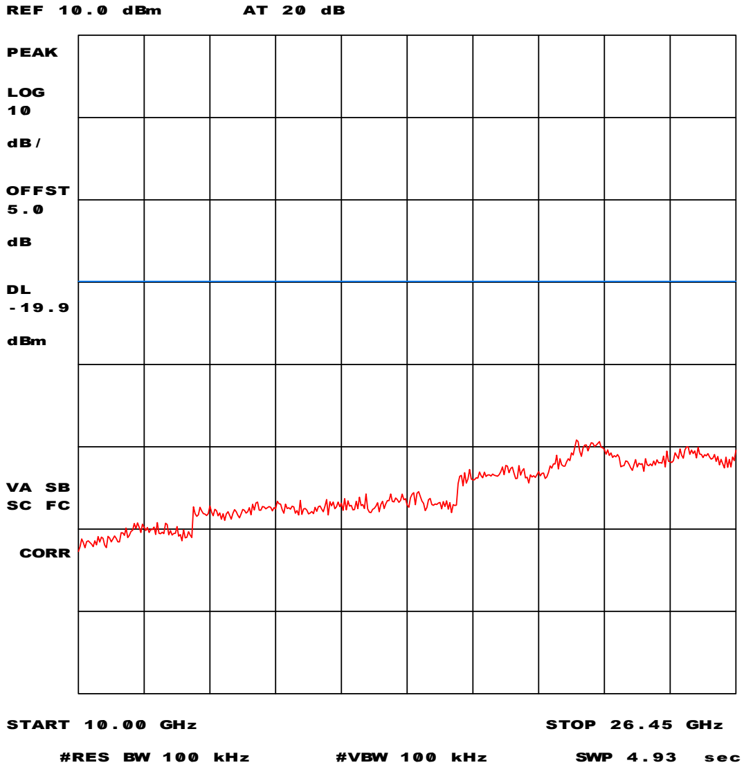
Plot 24 - Conducted emission outside restricted band (OFDM mode).
