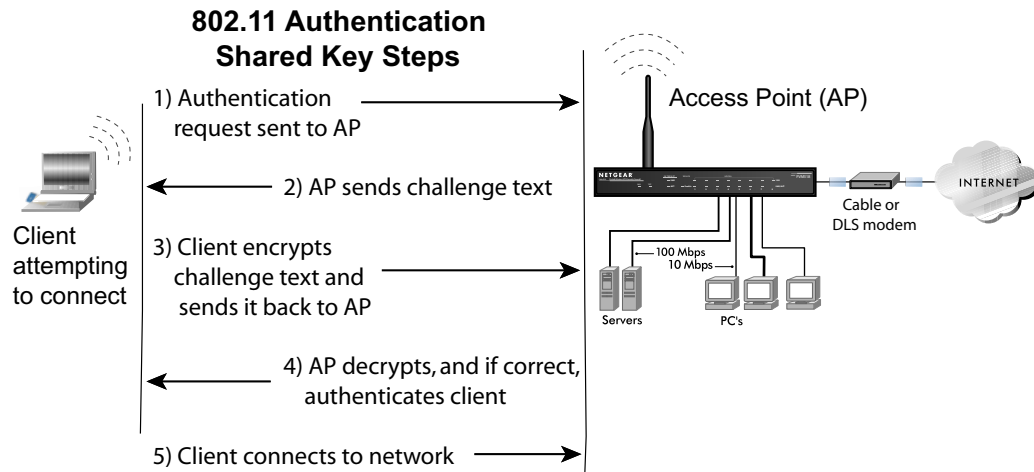
Figure B-2: 802.11 shared key authentication
