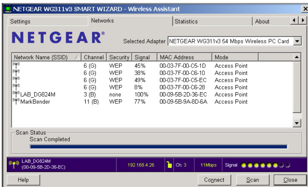
Figure 3-1: Networks tab page
