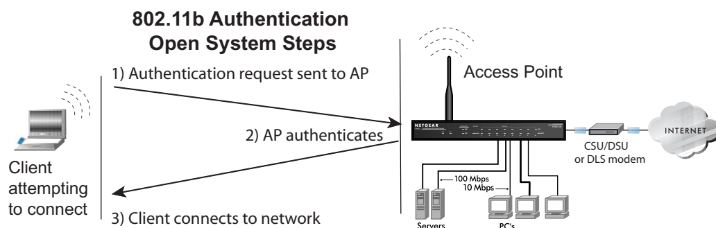
Figure B-1: 802.11 open system authentication
