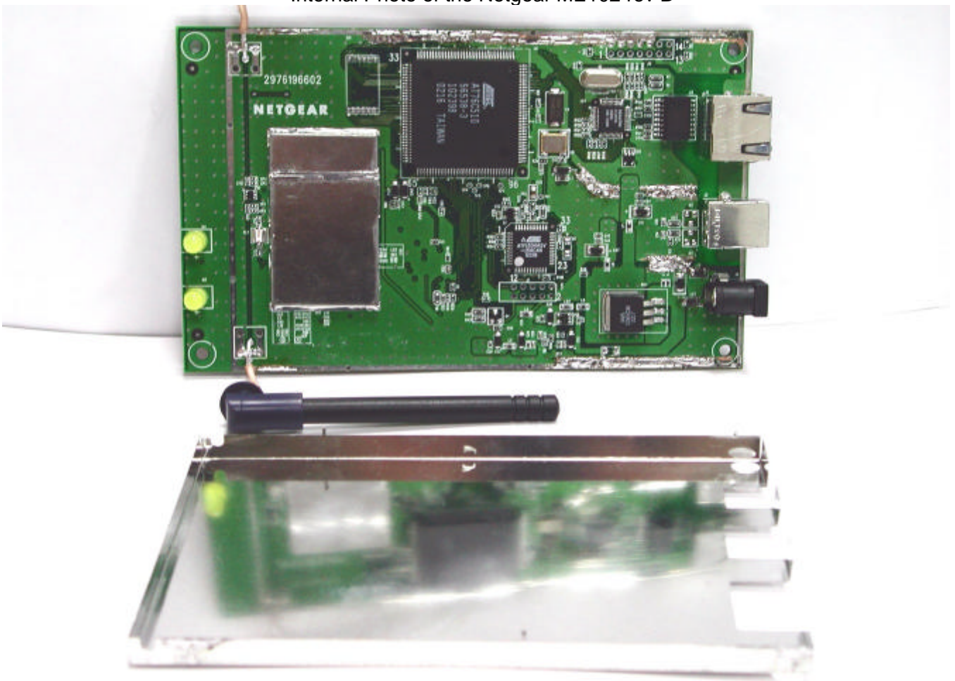
Internal Photo of the Netgear ME102 rev B
