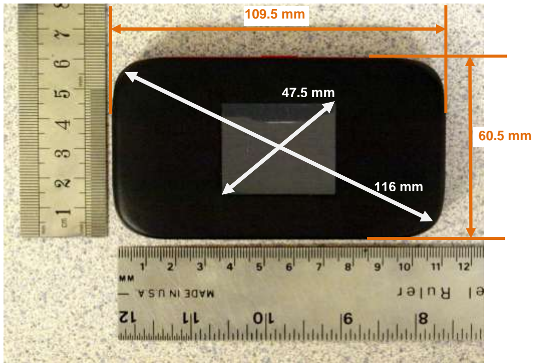
Overall Dimensions
