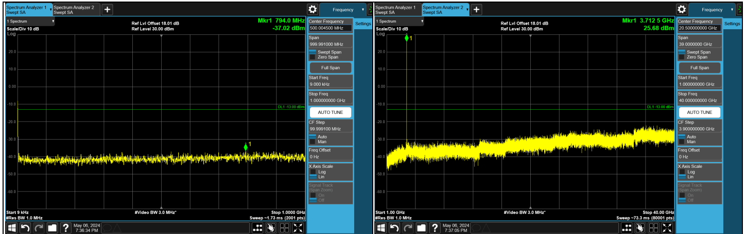
CH 647500 (3712.5 MHz)
