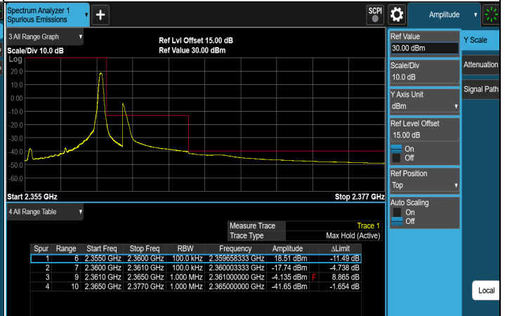
FULL CH 39225 (2357.5 MHz)
