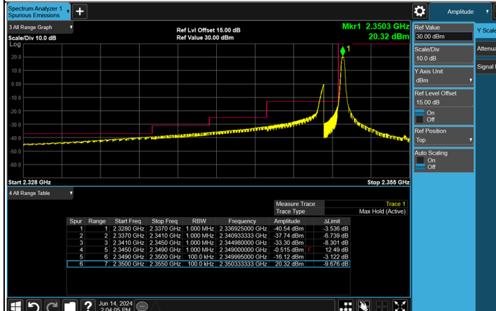
FULL CH 39175 (2352.5 MHz)
