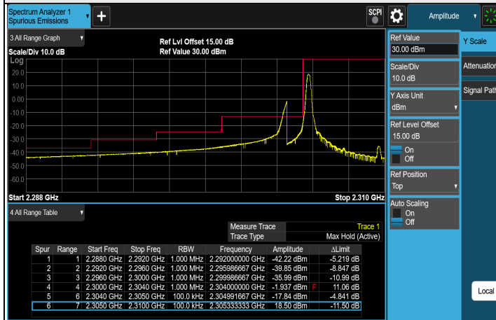
FULL CH 38725 (2307.5 MHz)
