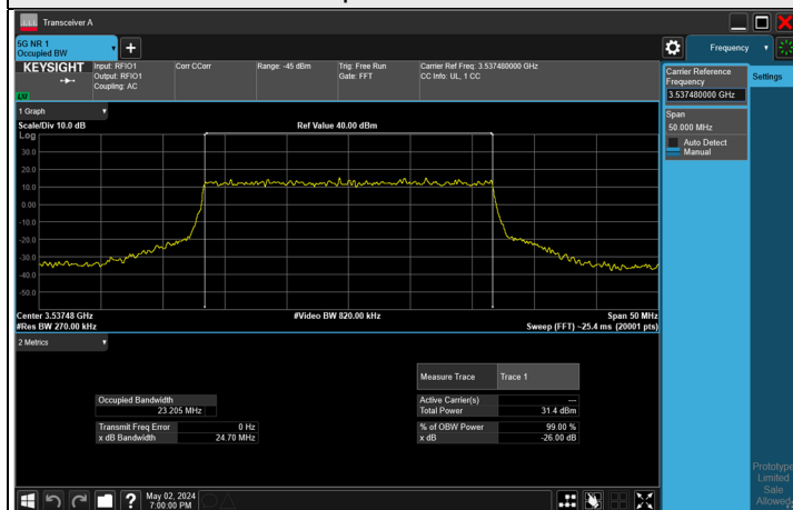
64QAM CH 635832 (3537.48 MHz)
