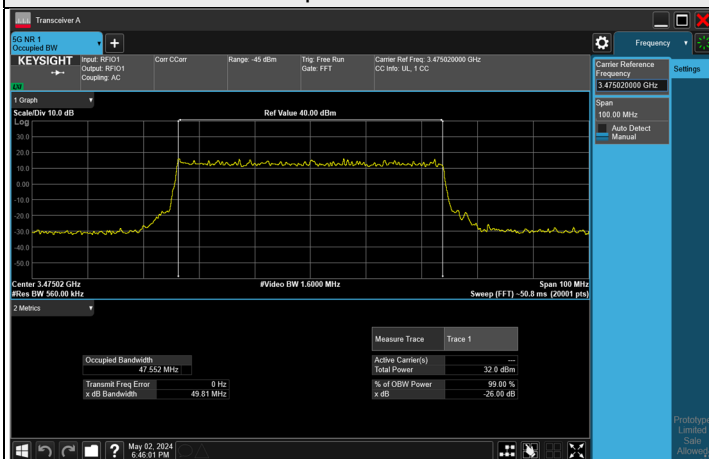
16QAM CH 631668 (3475.02 MHz)
