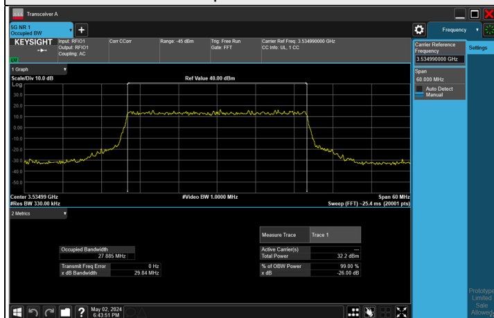
16QAM CH 635666 (3534.99 MHz)
