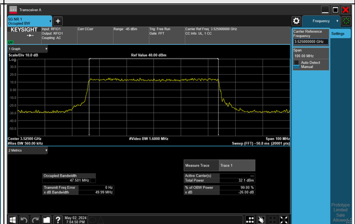
64QAM CH 635000 (3525 MHz)
