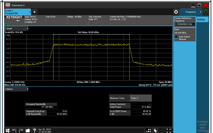
256QAM CH 648000 (3720 MHz)
