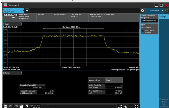
QPSK CH 647668 (3715.02 MHz)
