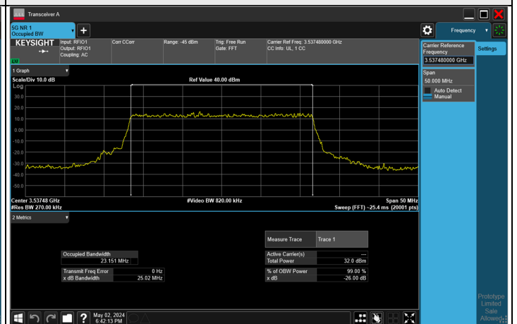
16QAM CH 635832 (3537.48 MHz)
