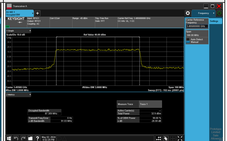
16QAM CH 633000 (3495 MHz)
