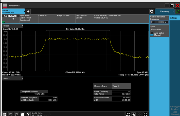
64QAM CH 647334 (3710.01 MHz)
