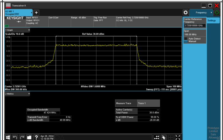
16QAM CH 648334 (3725.01 MHz)
