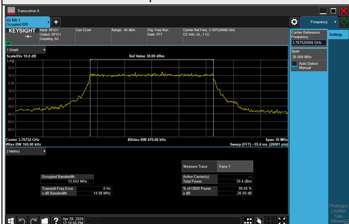
16QAM CH 647168 (3707.52 MHz)
