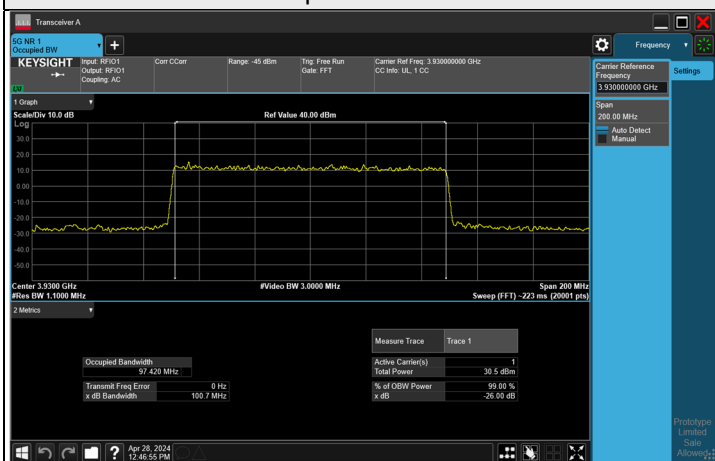
64QAM CH 662000 (3930 MHz)
