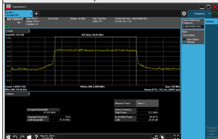
64QAM CH 632334 (3485.01 MHz)
