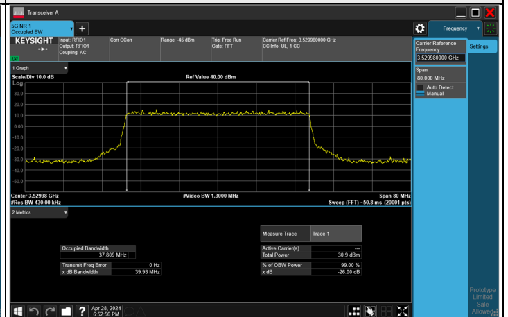
QPSK CH 635332 (3529.98 MHz)
