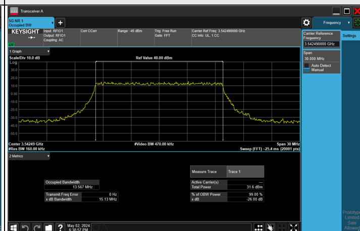
16QAM CH 636166 (3542.49 MHz)
