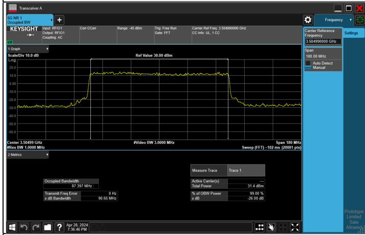
64QAM CH 633666 (3504.99 MHz)
