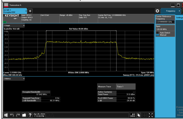
16QAM CH 634666 (3519.99 MHz)
