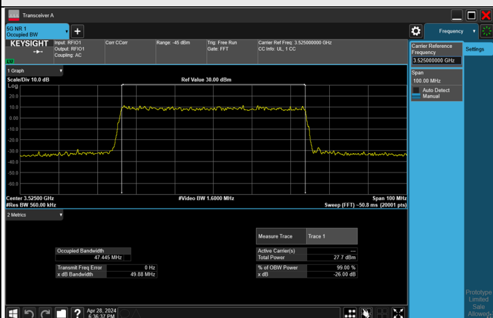
256QAM CH 635000 (3525 MHz)
