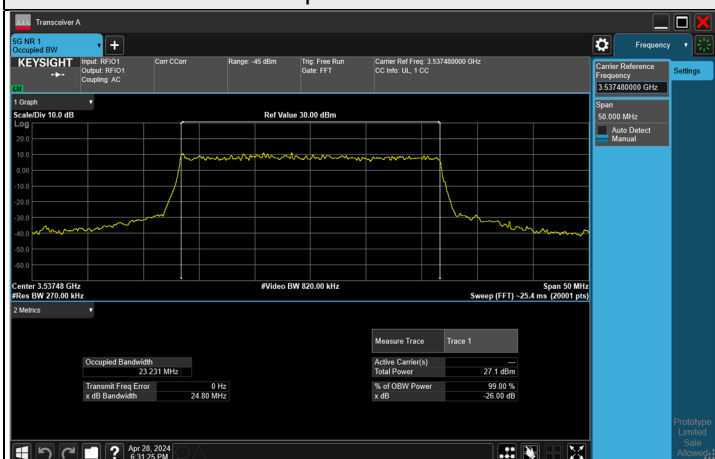
256QAM CH 635832 (3537.48 MHz)
