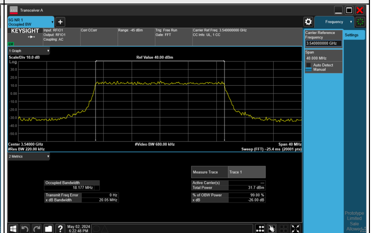
QPSK CH 636000 (3540 MHz)
