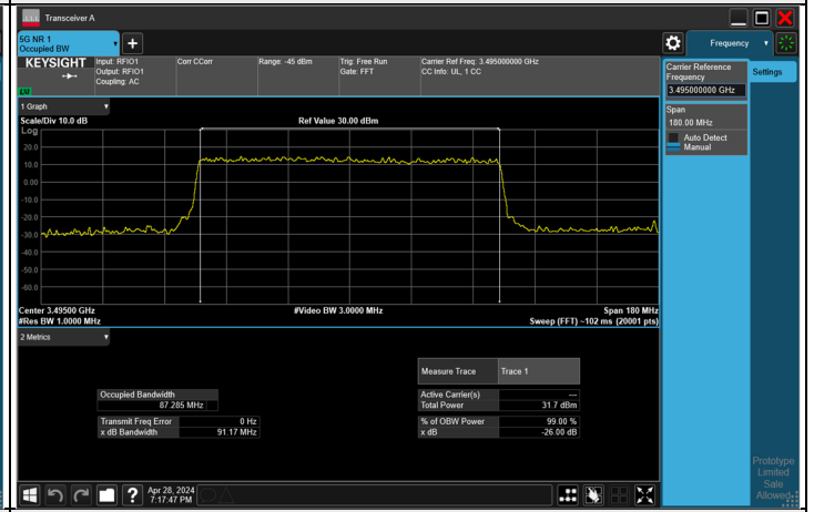
16QAM CH 633000 (3495 MHz)
