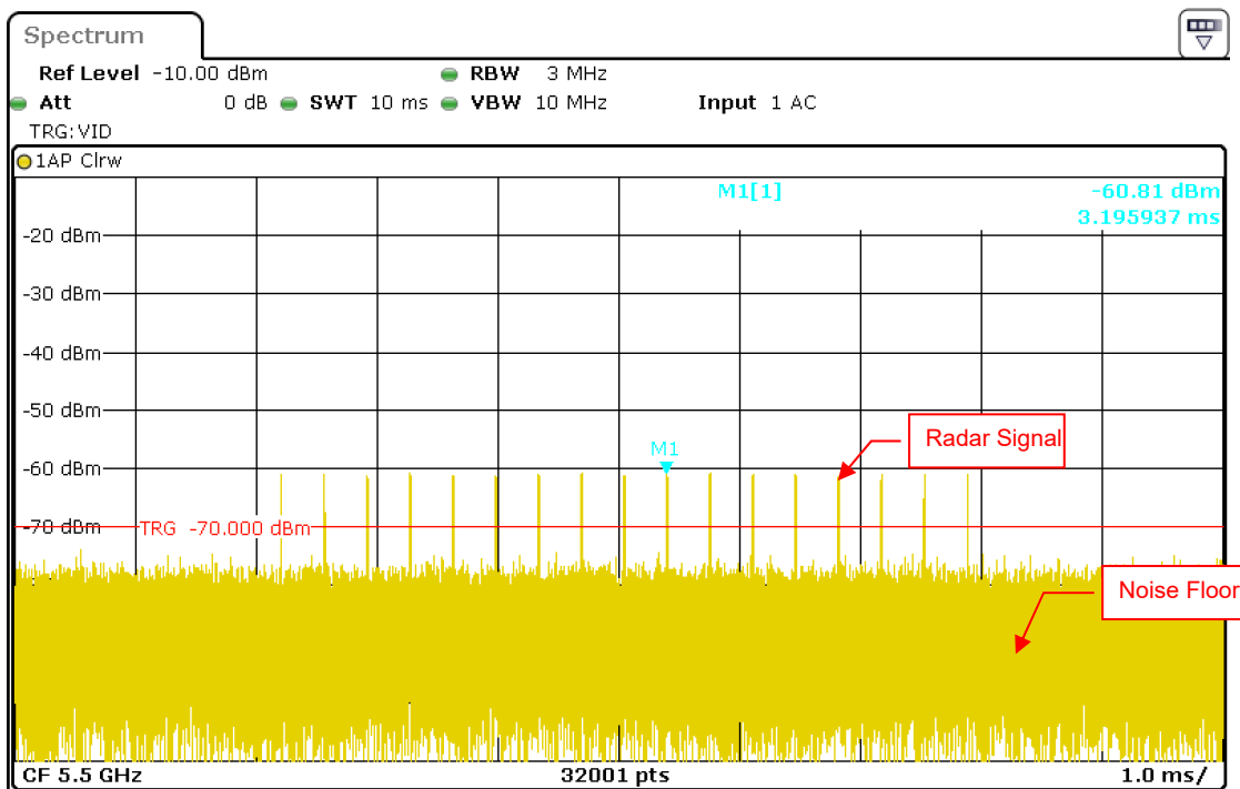
Radar Signal 3
