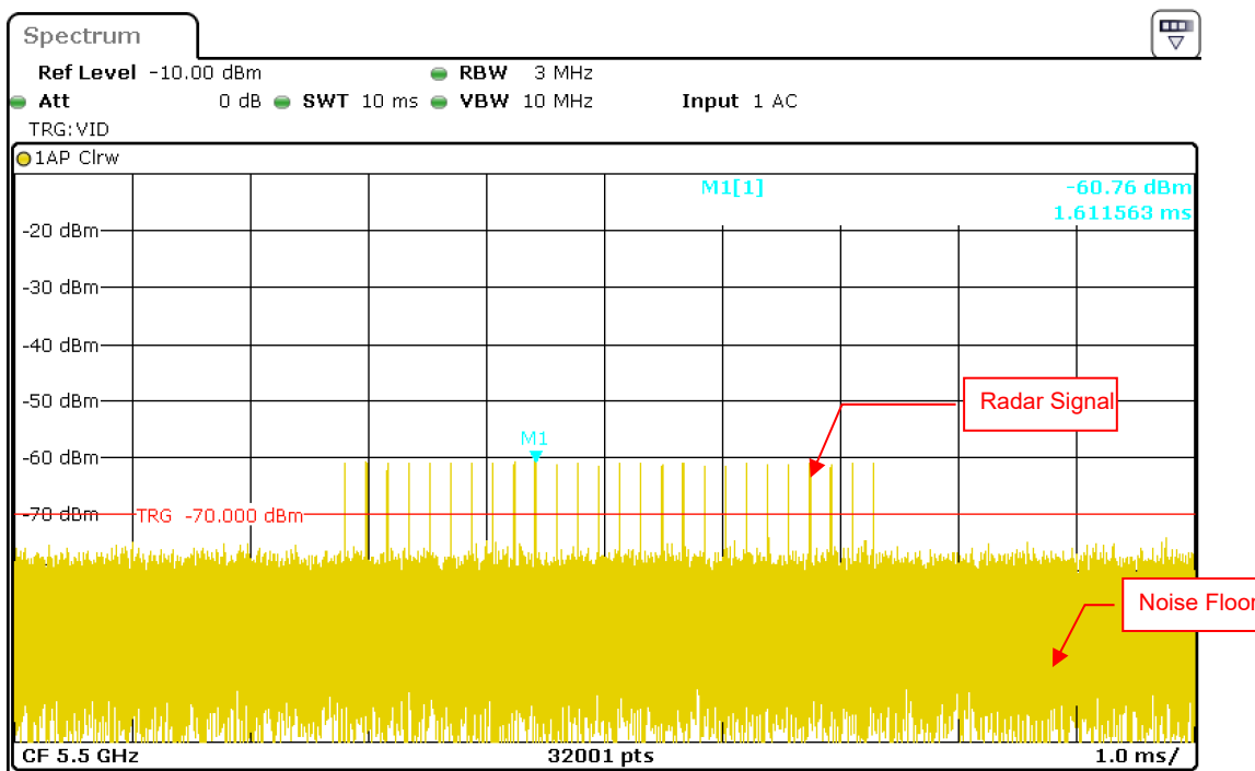
Radar Signal 2
