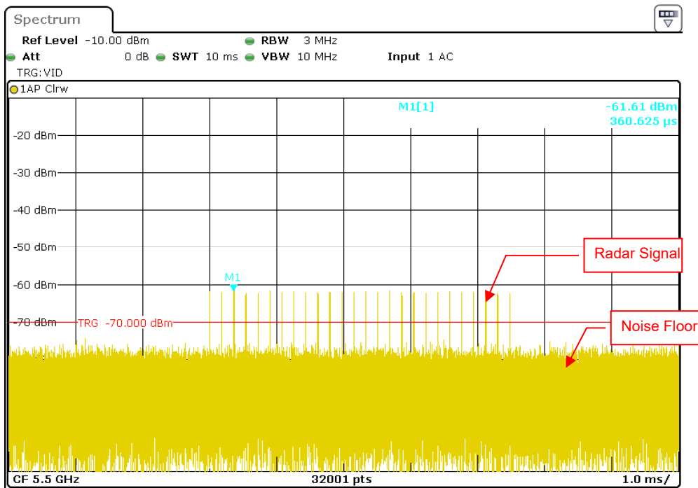
Radar Signal 2
