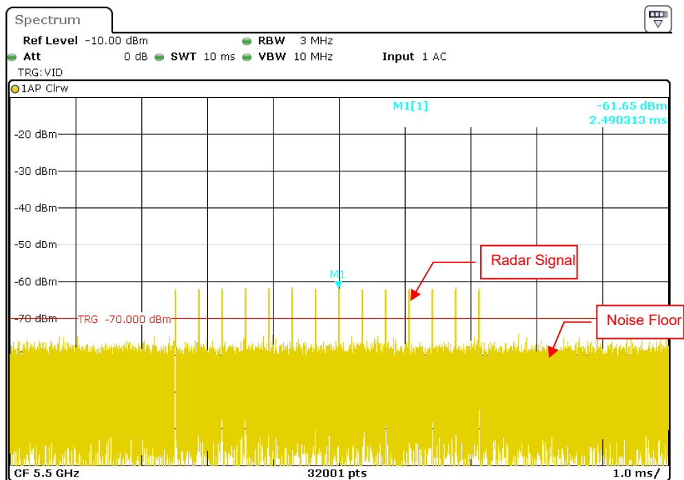
Radar Signal 4
