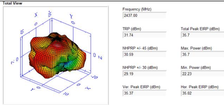
2.4GHz_HE20_CH6_BF On Nss1
