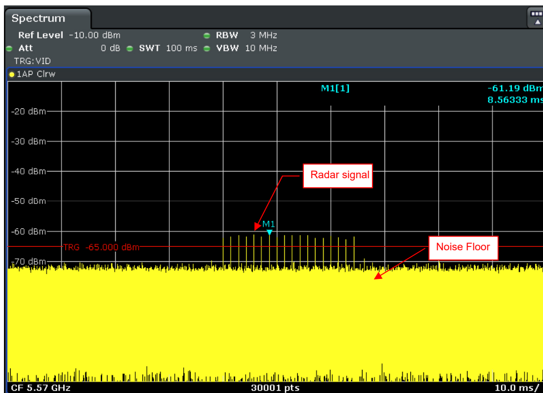
Radar Signal 0
