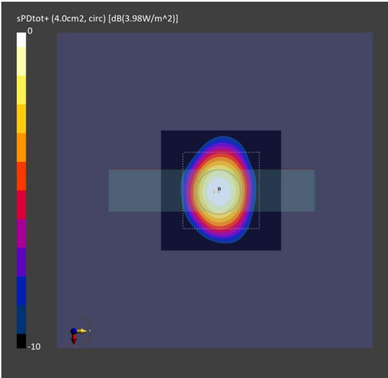
Figure8-3: 4cm 2 -averaged power density distribution measured at input.power.limit of 3.98dBm on the Left Side for n261 beam 39
