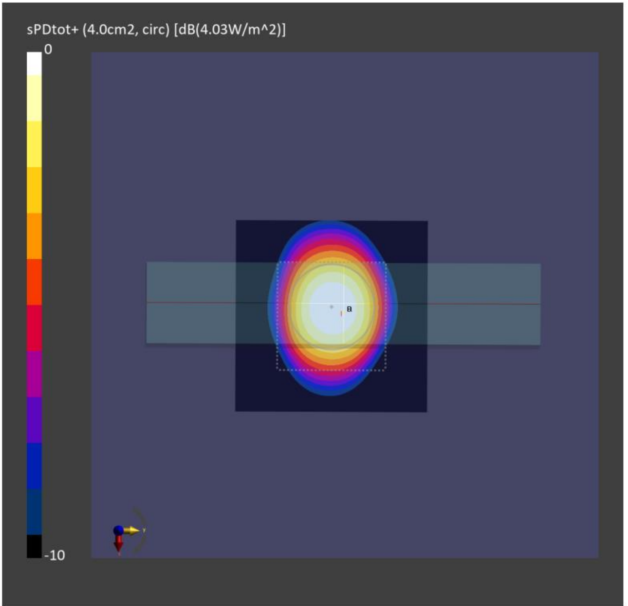
Figure8-2: 4cm 2 -averaged power density distribution measured at input.power.limit of 4.03dBm on the Right Side for n260 beam 36
