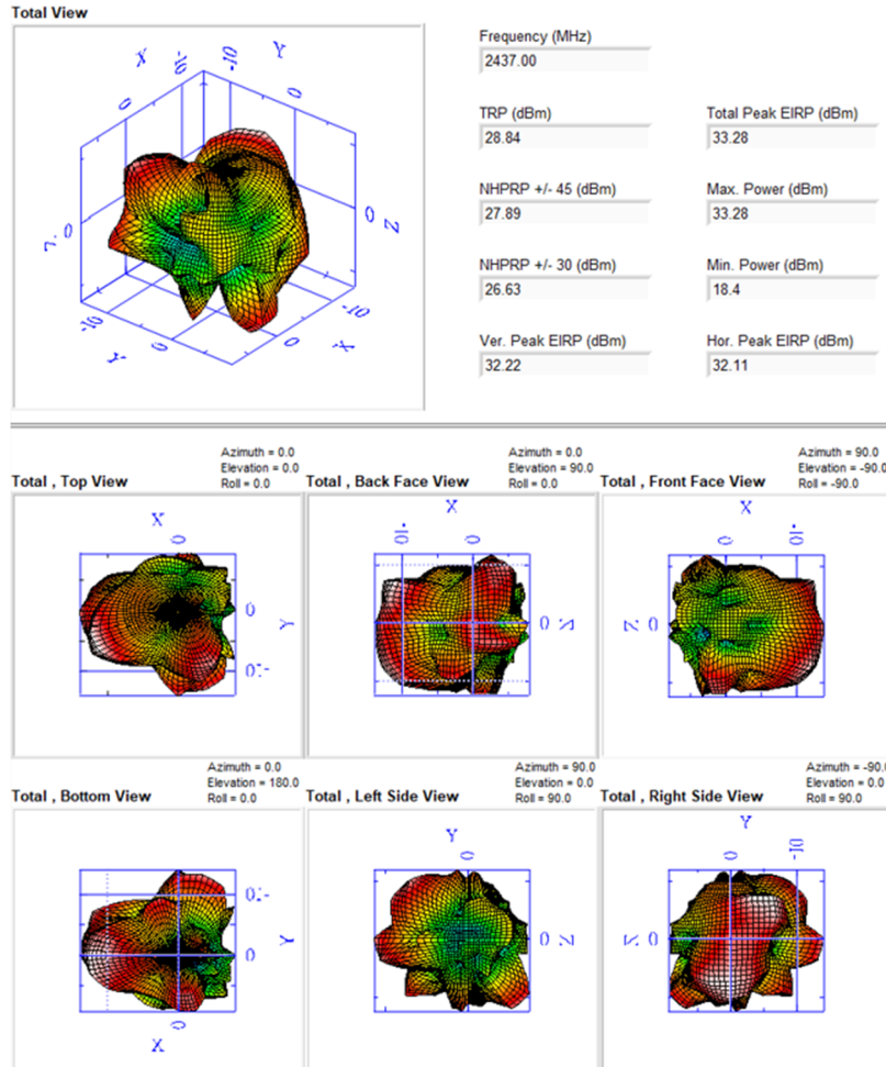
2.4GHz_HE20_CH6_BF On Nss1
