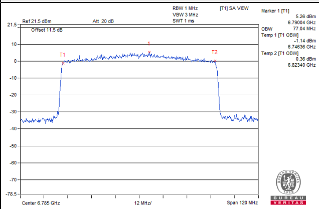
802.11ax (HE80)_Chain 0 / CH 167 (U-NII-7 Band)
