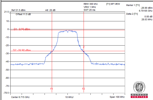
802.11a_Chain 0 / CH 153 (U-NII-7 Band)
