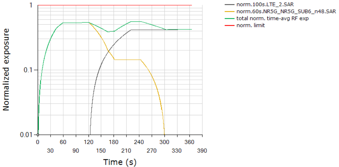
Total Normalized Time-averaged RF Exposure Tech: LTE, Band 2 / Tech: NR5G NR5G SUB6, Band n48
