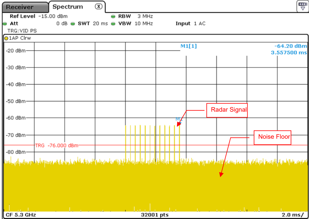
Radar Signal 4
