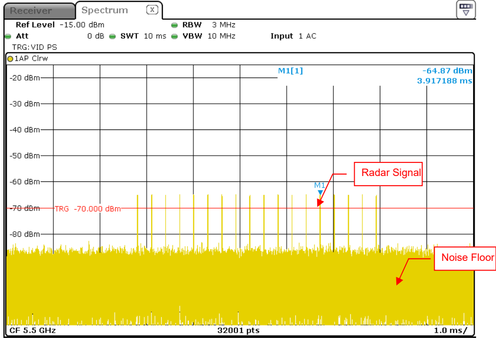
Radar Signal 3
