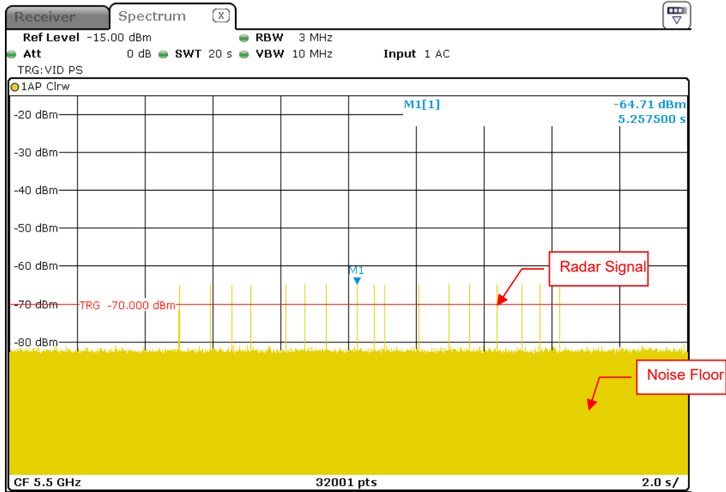
Radar Signal 5
